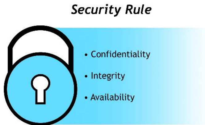
Figure 21.2 CIA Principle
