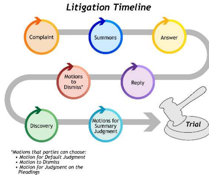
Figure 3.1 Litigation Flowchart
