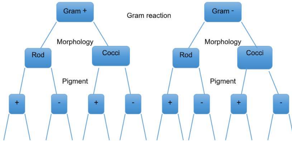
Figure 23.4.1: Flowchart to identify unknown bacteria
