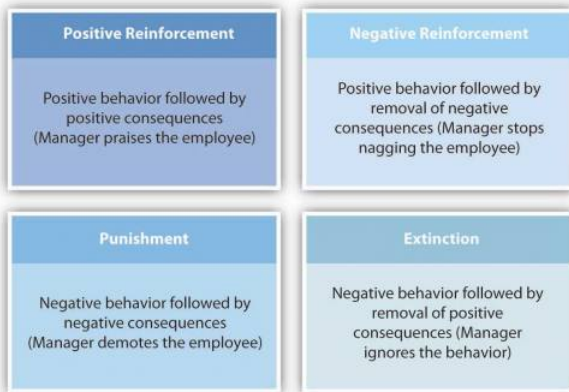
Figure 14.12 Reinforcement Methods
