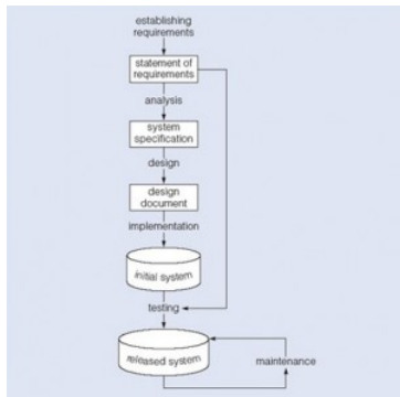
Figure 13.1. Waterfall model.
