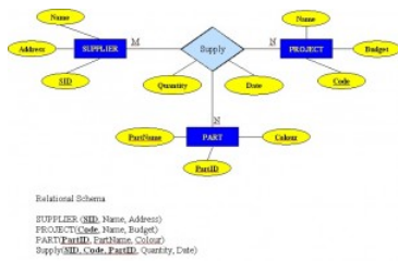
Figure 8.10. Example of a ternary relationship.
