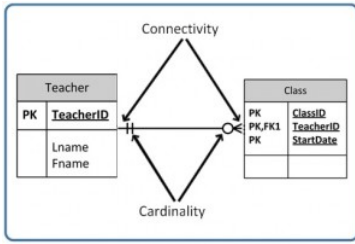
Figure 9.2. Position of connectivity and cardinality on a relationship symbol, by A. Watt.
