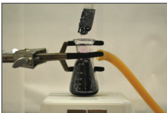
(D) Once the sublimation is complete, the cold finger is carefully removed.
