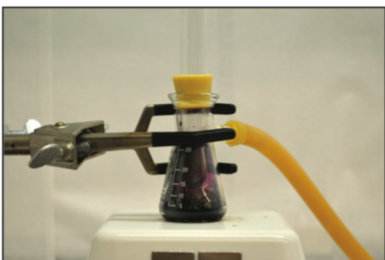
(C) As the temperature rises, more crude material sublimates. Inside the filter flask, the vapor reaches the cold finger.
