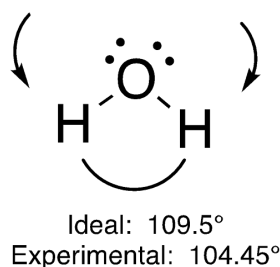
Figure 4. Efficient repulsion by the non-bonding electron pairs of water “squishes” the O – H bonds closer together than the idealized bond angle.
