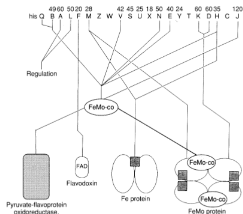
Figure 7.25 - Nif genes required for nitrogen fixation as arranged in Klebsiella pneumoniae , and their respective gene products. The numbers on the top are the molecular weights in kilodaltons of the respective gene products.
