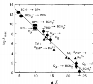
Figure 6.24 - Maximum electron-transfer rate ( k_{max} ) vs. edge-to-edge distance ( d ) for proteins. Photosynthetic reaction center rates are shown as circles and ^3\text{ZnP}^* to \text{Ru}^{3+} rates in modified myoglobins and cytochromes c are shown as triangles. Adapted from Reference 80.
