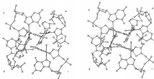
Figure 9.20 - Stereoview of aggregate of four cis -[Pt(NH 3 ) 2 {d(pGpG)}] molecules (reproduced by permission from Reference 130).
