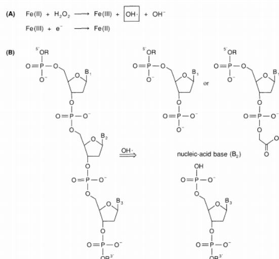
Figure 8.5 - An illustration of DNA strand cleavage mediated by hydroxyl radicals produced by the Fenton reaction (A) of \text{Fe(EDTA)}^{2-} with hydrogen peroxide. The cleavage scheme (B) shows the products obtained as a result of initial C4'-H abstraction by the hydroxyl radicals.
