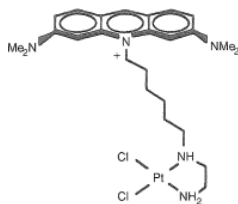
Figure 9.26 - Structure of AO-Pt in which the {Pt(en)C 12 } moiety is linked by a hexamethylene chain to acridine orange.
