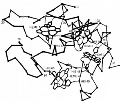
Figure 6.9 - Structure of cytochrome c_3 .
