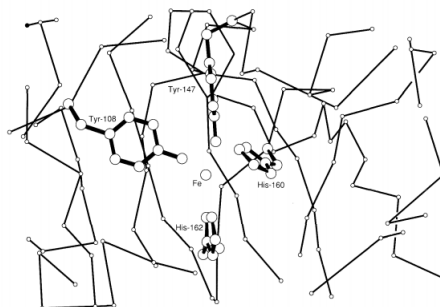
Figure 5.7 - A view of the active site of protocatechuate 3,4-dioxygenase based on the results of the x-ray crystal structure. 70 The Fe III center is approximately trigonal bipyramidal, with Tyr-147 and His-162 as axial ligands, and Tyr-108 and His-160 in the equatorial plane along with a solvent molecule (not shown) in the foreground. 66
