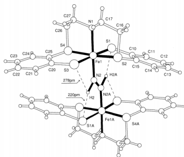
Figure 738 - The structure 338 of \text{FeL}(\text{N}_2)_2\text{FeL} ( \text{L} = \text{SC}_6\text{H}_4\text{SCH}_2\text{CH}_2\text{SCHCH}_2\text{SC}_6\text{H}_4\text{S} ).
