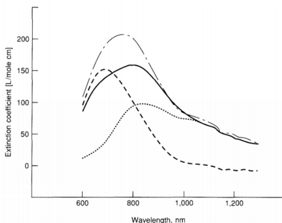
Figure 5.19 - Comparison of the visible absorption spectrum of CuCuSOD, -----, with that of CuZnSOD, ———, and of Ag I CuSOD, •••••. A digital addition of the spectra of CuZnSOD and of Ag I CuSOD generated the other spectrum, -•-•-•-. Note that the spectrum of CuCuSOD, which has Cu II ions in both the copper and the zinc sites, closely resembles a superposition of the spectra of CuZnSOD, which has Cu II in the copper site, and Ag I CuSOD, which has Cu II in the zinc site. (From M. W. Pantoliano, L. A. Nafie, and J. S. Valentine, J. Am. Chem. Soc. 104 (1982), 6310-6317.)
