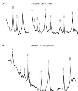
Figure 5.6 - Resonance Raman spectra of (A) Fe III (salen)(O - C 6 H 4 - 4 - CH 3 ) and (B) catechol 1,2-dioxygenase. 66
