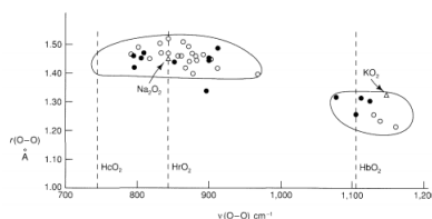
Figure 4.12 - Scatter diagram showing the distribution of O—O stretching frequencies and separations in ionic superoxides and peroxides ( \Delta ) and in coordination compounds. An open circle denotes O_2 coordinated to one metal; a filled circle denotes O_2 bridging two metals. The O—O stretching frequencies of oxyhemoglobin, oxyhemocyanin, and oxyhemerythrin are marked by dashed lines.
