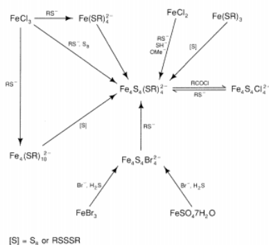
Figure 7.13 - Preparative schemes leading to complexes containing the Fe 4 S 4 core. 128
