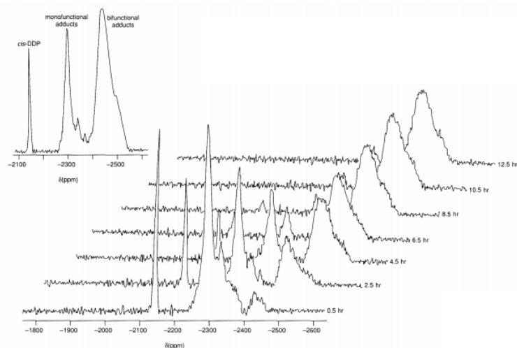
Figure 9.8 - Time course of the reaction between double-stranded chicken erythrocyte DNA and \text{cis-}[\text{Pt}(\text{NH}_3)_2(\text{H}_2\text{O})\text{Cl}]^+ at a D/N = 0.07 , in 3 mM NaCl and 1 mM \text{NaH}_2\text{PO}_4 , 37 °C, pH 6.5. Each spectrum consists of 200,000 transients. The inset shows the sum of the individual spectra (reproduced by permission from Reference 67).
