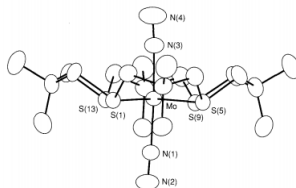
Figure 7.37 - The structure of Mo(N 2 ) 2 L (L is a tetrathiacyclohexadecane) 337b,c
