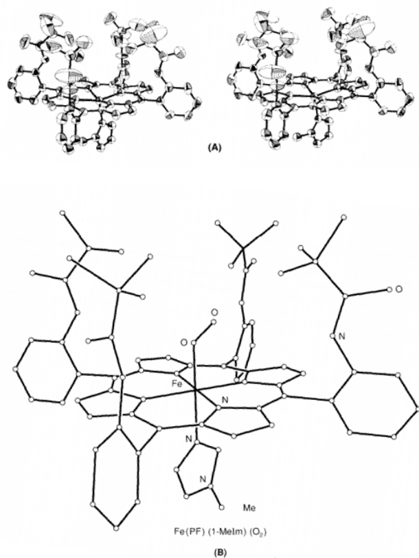
Figure 4.28 - (A) Stereodigram of the structure of Fe(PF)(2-MeIm). 172 (B) Structure of Fe(PF)(1-MeIm)(O 2 ). 187
