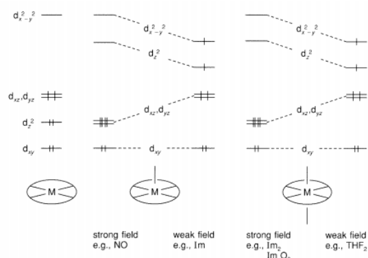
Figure 4.16 - d-Orbital splitting in metalloporphyrins as a function of number and ligand-field strength of ligands. 91 Orbital occupancy is illustrated for a d^6 species ( Fe^{II} or CO^{III} ).
