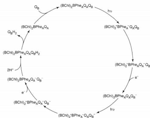
Figure 6.38 - Forward electron transfer through the reaction center. Note that two charge translocations must occur in order for the (labile) quinol Q_BH_2 to be produced. Once Q_BH_2 dissociates from the RC and is replaced by another, oxidized, Q_B , the cycle can begin anew.
