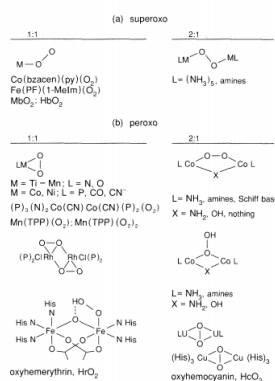
Figure 4.13 - Modes of attachment of O_2 to metals. P, N, and O denote phosphine, amine, and oxygen ligands, respectively.
