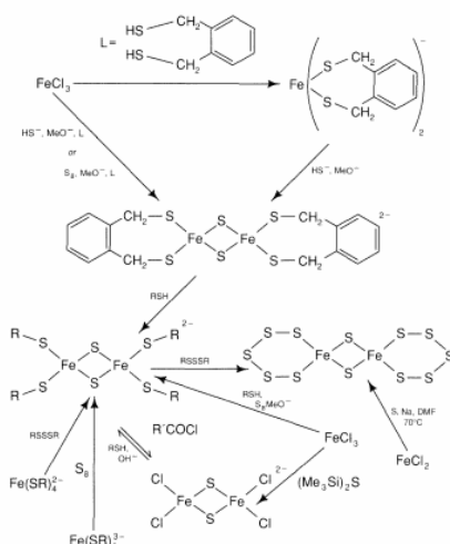
Figure 7.10: Preparative schemes leading to complexes containing the Fe_2S_2 core. 128
