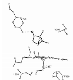
Figure 5.12 - Edge-on view of the P-450 active-site region with the substrate camphor molecule bound. 80 The substrate camphor is located in a hydrophobic pocket directly above the heme and is oriented by a hydrogen bond between the carbonyl oxygen of the camphor and Tyr-96. The position that is hydroxylated in the oxygenation reaction, i.e., the 5-exo position, is the closest point of approach of the substrate to the expected position of the oxygen atom bound to iron in the highvalent iron-oxo intermediate.
