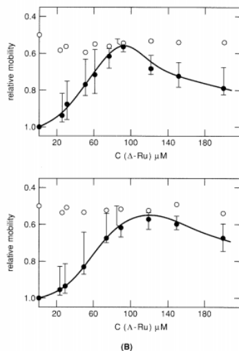
Figure 8.10 - The application of DNA supercoiling to probe metal-complex interactions with DNA. (A) A schematic representation of supercoiled DNA (form I), nicked DNA (form II) that, as a result of the single-strand scission, relaxes to a circular form lacking supercoils, and linear (form III) DNA. (B) Plots of the relative electrophoretic mobilities of form I (●) and form II (○) DNA as a function of increasing concentration of \Delta -(top) and \Lambda -(bottom) \text{Ru}(\text{phen})_3^{2+} in the gel. 46 Increasing concentrations of bound intercalator unwind the negatively supercoiled DNA. Given the higher intercalative binding affinity of the \Delta -isomer, slightly lower concentrations of this isomer are needed to unwind the plasmid to a totally relaxed state (where form I and II comigrate).
