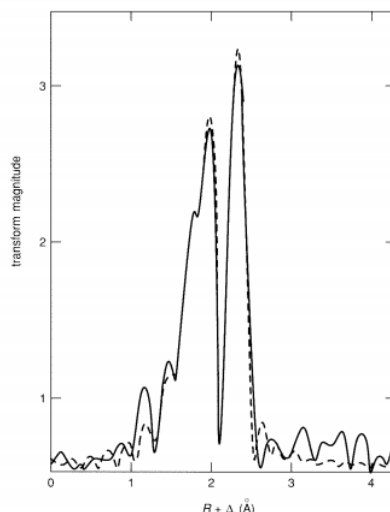
Figure 7.30 - Mo K-edge EXAFS spectrum (left panel) and EXAFS Fourier transform (right panel) of Klebsiella pneumoniae nitrogenase MoFe protein. The solid line is the processed experimental spectrum and the dashed line a calculated one. 287
