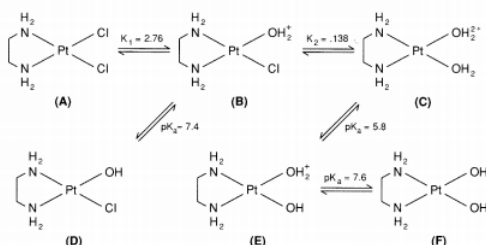
Figure 9.7 - Hydrolysis reactions of antitumor platinum complexes and an estimate of the species present in plasma and cytoplasm (reproduced by permission from Reference 51).
