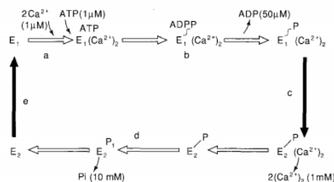
Figure 3.12 - Simplified schematic reaction cycle of the \text{Ca}^{2+} -ATPase of sarcoplasmic reticulum (SR). 49,51 The transport protein is assumed to be in either of two states, E_1 on the cytoplasmic side, or E_2 on the side of the SR lumen. Starting from E_1 in the upper left corner, the reactions steps shown are: (a) binding of \text{Ca}^{2+} and ATP (approximate dissociation constants within parentheses); (b) rapid phosphorylation of Asp-351 of the protein ( E_1\text{-P} ) and release of ADP; (c) transformation from an energy-rich, high- \text{Ca}^{2+} -affinity conformation ( E_1\text{-P} ) ( \text{Ca}^{2+} ) 2 to a low-energy, low-affinity conformation ( E_2\text{-P} ) ( \text{Ca}^{2+} ) 2 ; (d) hydrolysis of the phosphorylated protein and release of the phosphate into the lumen; (e) return to the original state.
