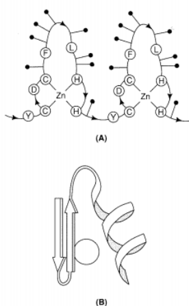
Figure 8.17 - (A) A schematic of a zinc-finger peptide domain. 82 (B) The proposed schematic structure of a zinc-finger domain based on comparisons to other structurally characterized metalloproteins. 85
