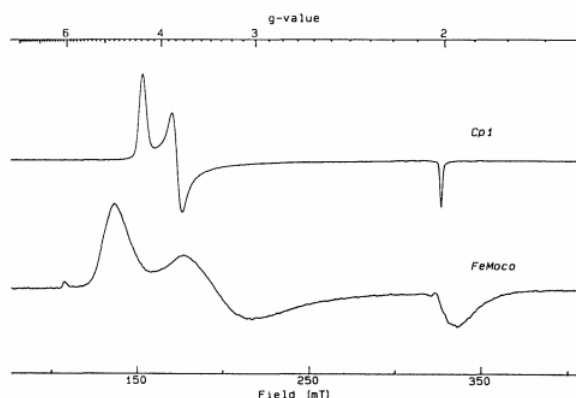
Figure 7.28: EPR spectra: (A) the S = \frac{3}{2} M center in Clostridium pasteurianum nitrogenase FeMo protein; and (B) the FeMoco extracted into NMF from the protein. (Spectra courtesy of R. Bare and G. N. George.)
