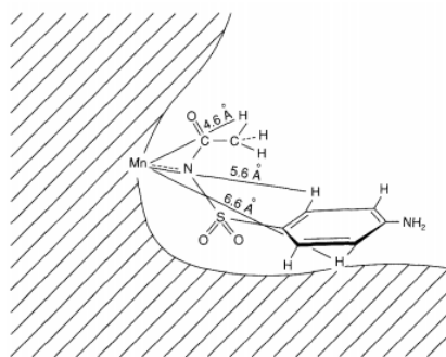
Figure 2.19 - Schematic drawing of the geometric arrangement of the inhibitor N-acetyl-sulfanilamide in the active cavity of manganese(II)-substituted CA, as revealed by ^1\text{H} NMR spectroscopy. 92
