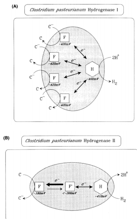
Figure 7.22 - Redox schemes illustrating proposed action of Fe hydrogenases: (A) Clostridium pasteurianum hydrogenase I; (B) Clostridium pasteurianum hydrogenase II. 189a,199
