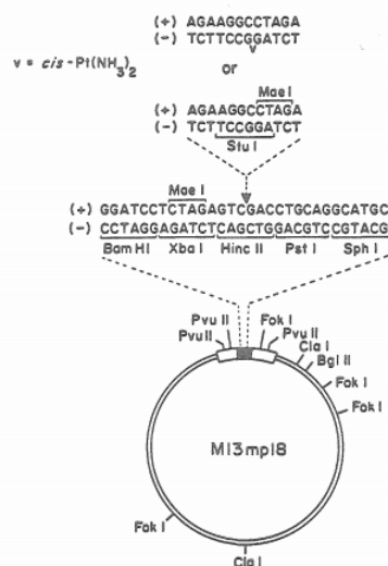
Figure 9.29 - Map of the genome created by insertion of cis -DDP platinated or unplatinated d(TpCpTpApGpGpCpCpTpTpCpT) \cdot d(ApGpApApGpGpCpCpTpTpApGpA) into the Hinc II restriction site of bacteriophage M13mp18 DNA.
