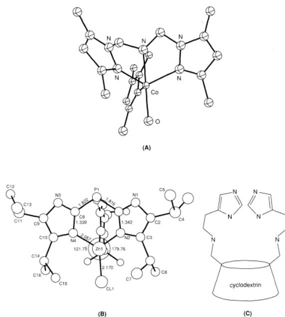
Figure 2.25 - Some multidentate ligands as models of CA: (A) tris-(3,5-dimethyl-1-pyrazolylmethyl) amine 4 (cobalt[II] complex); (B) tris (4,5- diisopropylimidozal-2yl)phosphine 104 (zinc[II] complex); (C) bis(histamino) \beta -cyclodextrin.
