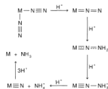
Figure 7.36 - Structure and reactions of M(N 2 ) 2 (Ph 2 PCH 2 CH 2 PPh 2 ) 2 (M = Mo, W) and related complexes. Not all of the intermediates in this scheme have been isolated in anyone particular system. 336,337,337a The phosphine ligands are not shown.
