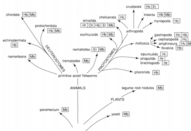
Figure 4.8 - Phylogenetic distribution of oxygen-carrier proteins: Hb, hemoglobin; Mb, myoglobin; Er, erythrocrurin; Ch, chlorocruorin; He, hemocyanin; Hr, hemerythrin. 15a Reproduced with permission from K. E. van Holde and K. I. Miller, Quart. Rev. Biophys. 15 (1982), 1-129.
