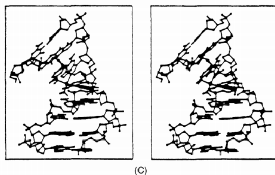
Figure 9.22 - (A) Stereoscopic view of the unkinked, platinated model of duplex d(\text{TpCpTpCpG}^*\text{pG}^*\text{pTpCpTpC}) from molecular-mechanics calculations. Counter ions used to stabilize the negative charge of the phosphates are not shown. (B) Stereoscopic view of the "high-salt" kinked, platinated model of duplex d(\text{GpGpCpCpG}^*\text{pG}^*\text{pCpC}) from molecular-mechanics calculations. Counter-ions are not depicted, with the exception of the bridging ion. (C) Stereoscopic view of the "low-salt" kinked, platinated model of duplex d(\text{GpGpCpCpG}^*\text{pG}^*\text{pCpC}) . Counter-ions are not depicted. Reproduced with permission from Reference 133.
