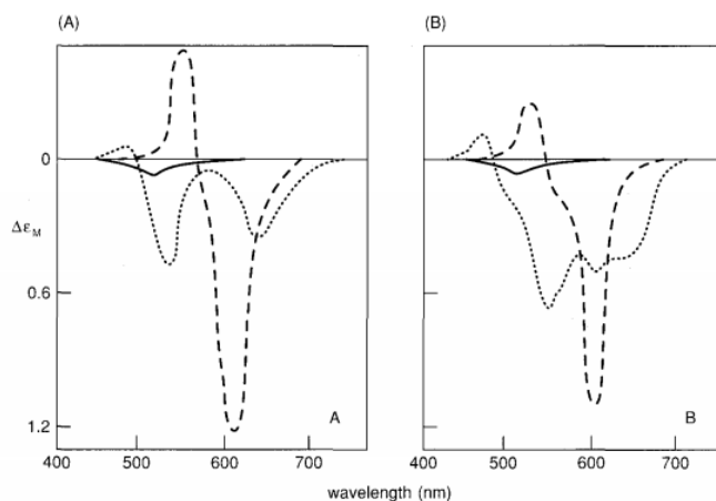
Figure 2.11 - (A) MCD spectra of model six-coordinate (Co(Gly-Gly) 2 , —), five-coordinate ((CoMe 6 tren)Br 2 , . . . . , and four-coordinate (Co(py) 2 Br 2 , ---) cobalt(II) complexes and (B) MCD spectra of the cobalt(II) derivatives of pyruvate kinase (—), alkaline phosphatase (••••), and carbonic anhydrase in the presence of acetazolamide (---). 21,61
