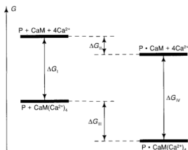
Figure 3.19 - Scheme depicting the standard free energies of different states in a system consisting of \text{Ca}^{2+} , calmodulin (CaM), and a target protein (P). \text{P}\cdot\text{CaM} denotes a complex between calcium-free CaM and P, \text{P}\cdot\text{CaM}(\text{Ca}^{2+})_4 denotes a complex with \text{Ca}^{2+} -loaded CaM. If the affinity of the \text{Ca}^{2+} -loaded CaM with the target protein P is higher than that of the \text{Ca}^{2+} -free form—i.e., |\Delta G_{\text{III}}| > |\Delta G_{\text{II}}| —it follows that the \text{Ca}^{2+} affinity of the complex p. CaM is higher than that of CaM itself.
