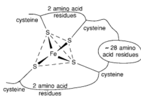
Figure 1.5 - Fe 3+/2+ coordination in rubredoxin.
