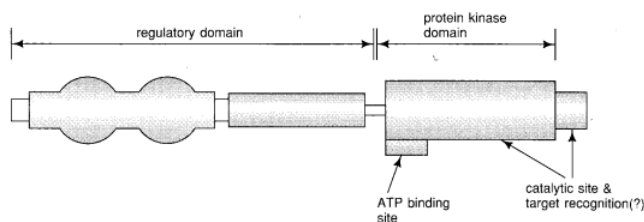
Figure 3.28 - Schematic representation of the structure of rabbit protein kinase C. 138 Three highly homologous protein kinases C were actually identified with M r ≈ 76,800. The kinase region shows clear similarity with other kinases. The regulatory domain should contain binding sites for Ca 2+ , phosphatidyl serine (PS), and diacylglycerol (DG).
