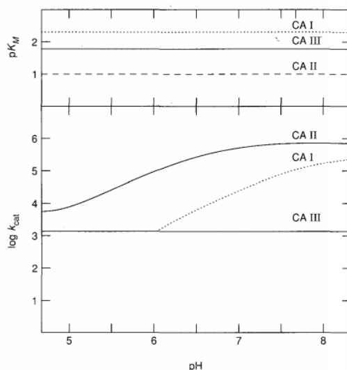
Figure 2.2 - pH dependence of k_{cat} and K_m values for \text{CO}_2 hydration catalyzed by carbonic anhydrase I, II, and III isoenzymes. 33,36
