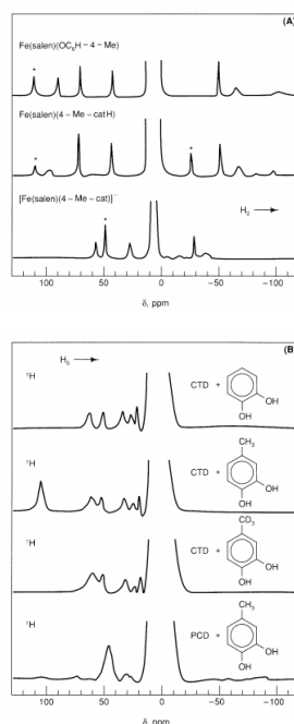
Figure 5.8 - (A) Paramagnetically shifted 1 H-NMR spectra of Fe(salen) complexes with 4-methylphenolate and 4-methylcatecholate ligands. Starred resonances are assigned to methyl groups. The top spectrum is of the ferric-salen complex of the monodentate 4-methylphenolate ligand. The middle spectrum is of the ferric-salen complex of the monoprotonated 4-methylcatecholate ligand. Note that two isomers are present, because the two oxygen atoms on the ligand are inequivalent, and either may be used to make the monodentate complex. The bottom spectrum is of the ferric-salen complex of the fully deprotonated 4-methylcatecholate ligand, which binds to the iron in a bidentate fashion. Note the smaller span of isotropic shifts, which has been demonstrated to be diagnostic of bidentate coordination. (B) Paramagnetically shifted 1 H-NMR spectra of enzyme-substrate complexes of the dioxygenase enzymes catechol 1,2-dioxygenase (CTD) and protocatecholate 3,4-dioxygenase (PCD). Note the resemblance between the position of the methyl resonance in the complex of 4-methylcatechol with CTD and that of one of the methyl resonances in the middle spectrum in (A), indicating that 4-methylcatechol binds to the ferric center in CTD in a monodentate fashion through the O-1 oxygen only. By contrast, the spectrum of 4-methylcatechol with PCD resembles the bottom spectrum in (A), indicating that here the 4-methylcatecholate ligand is bidentate. 66
