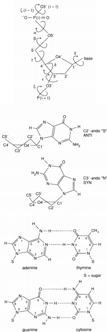
Figure 9.9 - Structural components of DNA. The left panel shows a schematic of the DNA backbone, including the deoxyribose ring numbering scheme and torsion angles. The center panel gives the two main classes of sugar pucker and base orientations. The right panel gives the bases in their Watson-Crick, A-T, and G-C pairs and the base numbering scheme, viewed down the helix axis, with the major grooves pointing toward the top of the figure and the minor grooves toward the bottom.
