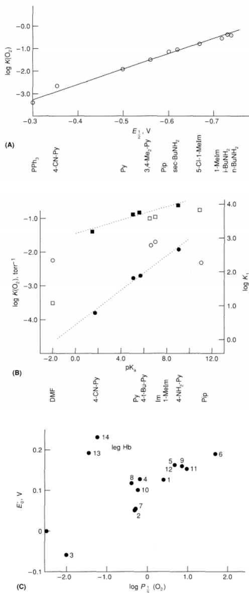
Figure 4.18 - Linear free-energy relationships: (A) Correlation of the O 2 affinity at -21 °C of Co(bzacen)L with the CO III ⇌ CO II cyclic voltammetric wave of Co(bzacen)L 2 species, 104a (B) Correlation of ligand affinity with pK a . Squares (□) pertain to the binding of L to Co(PPIX) at 23 °C. Circles (○) pertain to the O 2 affinity at -45 °C of Co(PPIX)L species, Filled shapes pertain to substituted pyridines; the least-squares lines shown are calculated from these data only, 104a (C) Correlation of E 0' (from cyclic voltammetry) with affinity for a miscellany of hemoglobins: 108 1, Aphysia limacina Mb; 2, Physeter macrocephalus Mb; 3, Candida mycoderma Hb; 4, Chironomus thummi Hb; 5, Hb M -Hyde Park; 6, Hb M -Iwate; 7, Hb α chain; 8, Hb β chain; 9, Hb F; 10, Hb γ chain; 11, HbA; 12, Glycera dibranchiata ; 13, legHb-a; 14, legHb-c, Reproduced with permission from A. W. Addison and S. Burman, Biochim. Biophys. Acta 828 (1985), 362-368.
