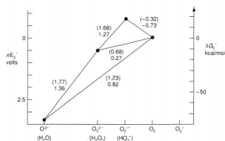
Figure 4.11 - Free-energy changes in the aqueous redox chemistry of dioxygen. Standard state P(O_2) = 1 . Electrode potentials are at pH 7; those in parentheses are at unit activity.
