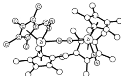
Figure 7.34 - The x-ray crystal structure 333 of (Cp) 2 Zr(N 2 )( \mu_2 -N 2 )Zr(N 2 )(Cp) 2 .
