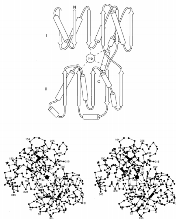
Figure 1.11: Three-dimensional structure of lactoferrin. Top: schematic representation of the folding pattern of each lactoferrin lobe; Domain I is based on a beta-sheet of four parallel and two antiparallel domains; Domain II is formed from four parallel and one antiparallel strand. Bottom: stereo Ca diagram of the N lobe of lactoferrin; (●) iron atom between domain I (residues 6 - 90+) and domain II (residues 91 - 251); (■) disulfide bridges; (★) carbohydrate attachment site. See Reference 39.
