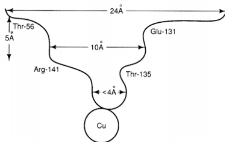
Figure 5.17 - Schematic diagram of a cross section of the active-site channel in CuZnSOD. The diameter of the channel narrows as the Cu II center is approached, and only small ligands can actually reach that site. In addition to the positively charged Cu II ion at the bottom of the channel, the positively charged side chain of Arg-141 is part of the walls of the channel. Two positively charged lysine side chains, not shown in this diagram, are close to the mouth of the channel. (From E. D. Getzoff, R. A. Hallewell, and J. A. Tainer, in M. Inouye, ed., Protein Engineering: Applications in Science, Industry, and Medicine , Academic Press, 1986, pp. 41-69.)
