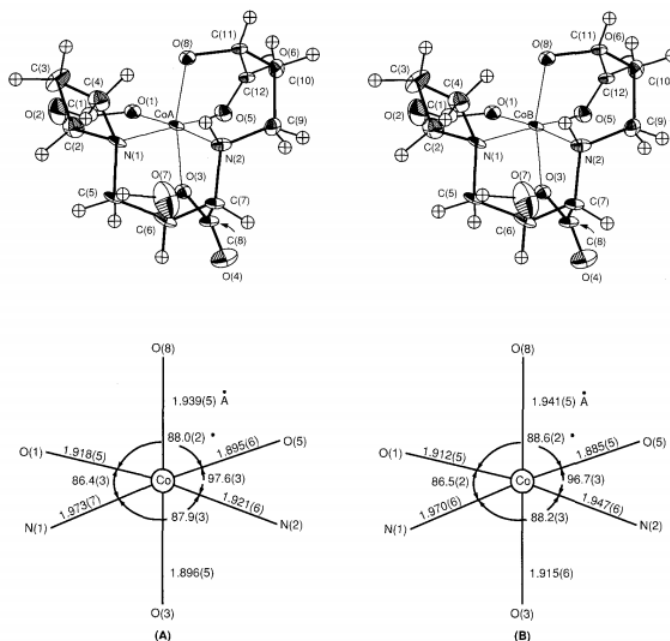
Figure 1.18 - Molecular structures of the complexes (molecules A and B) and coordination about the cobalt ion in molecules A and B of the mugenic acid-Co(III) complex. Bond lengths in Å; angles in degrees. See Reference 42.
