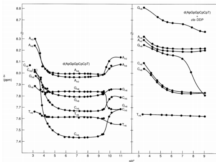
Figure 9.19 - Chemical shift ( \delta ) vs. pH^* of the nonexchangeable base protons of D_2O solutions of [d(ApGpGpCpCpT)]_2 (3.5 mM, 35 °C) and its cis -DDP adduct (2.5 mM, 70 °C). The pyrimidine resonances of the latter sample show no chemical shift changes with temperature over the range 35 < T < 70 °C while the purine resonances show a slight temperature-dependent chemical shift change of up to 0.1 ppm. Tetramethylammonium chloride was used as the internal standard ( \delta 3.180). Reproduced by permission from J. C. Caradonna, S. J. Lippard, M. J. Gait, and M. Singh, J. Am. Chem. Soc. 104 (1982), 5793.
