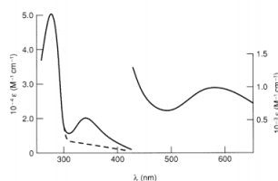
Figure 4.20 - Spectral changes accompanying oxygenation of hemocyanin: deoxyhemocyanin (---); oxyhemocyanin (—). 5 Reproduced with permission from A. G. Sykes, in A. G. Sykes, ed., Advances in Inorganic and Bioinorganic Mechanisms , Academic Press, 1 (1985), 121-178.
