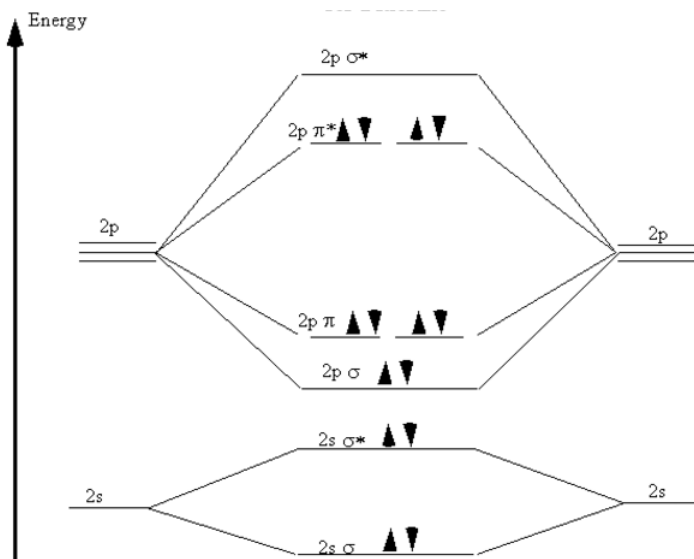
Figure 9.6: Molecular orbital energy diagram for fluorine.
