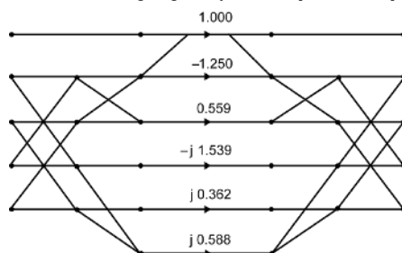
Fig. 6.2.1 Flow Graph for the Length-5 DFT
