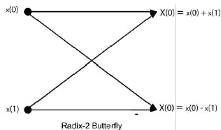
Fig. 8.2.1 A Radix-2 Butterfly
