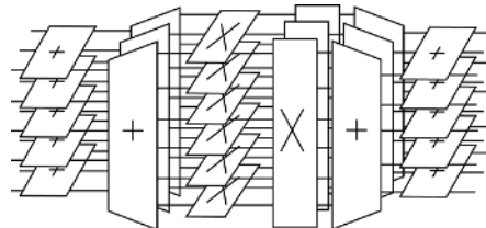
Fig. 9.3.1 A Length-15 WFTA with Nested Multiplications
