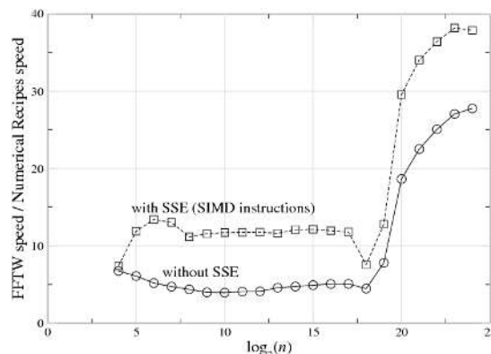
Fig. 10.1.1 The ratio of speed (1/time) between a highly optimized FFT (FFTW 3.1.2) and a typical textbook radix-2 implementation (Numerical Recipes in C on a 3 GHz Intel Core Duo with the Intel C \geq 2^{19} , the ratio increases because the textbook code becomes much slower (this happens when the DFT size exceeds the level-2 cache).
