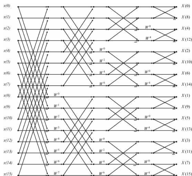
Fig. 14.1.1 Length-16, Decimation-in-Frequency, In-order input, Radix-2 FFT
