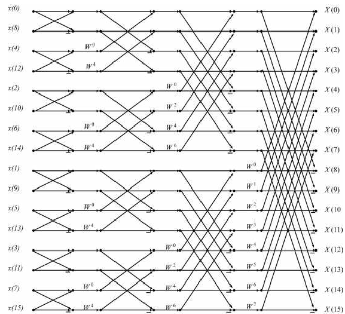
Fig. 14.1.2 Length-16, Decimation-in-Frequency, In-order output, Radix-2 FFT
