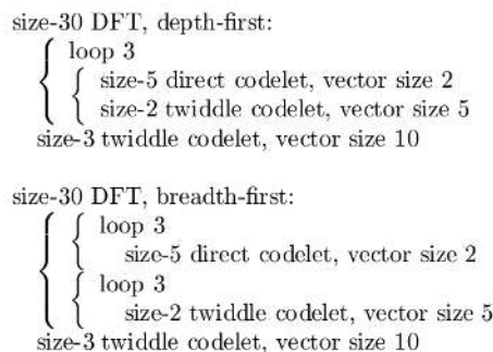
Fig. 10.5.1 Two possible decompositions for a size-30 DFT, both for the arbitrary choice of DIT radices 3 then 2 then 5, and prime-size codelets. Items grouped by a "Math input error" result from the plan f
