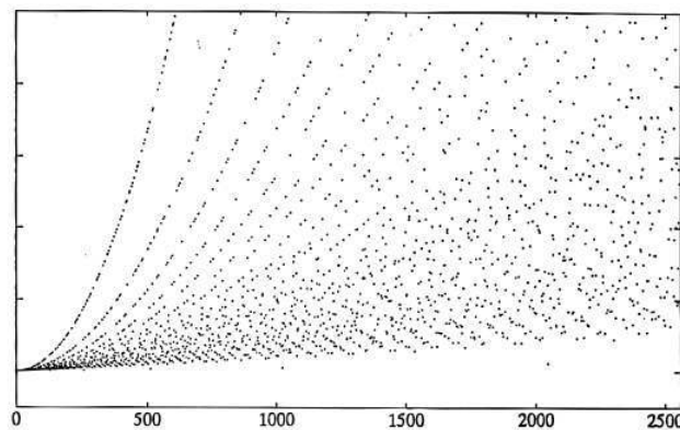
Fig. 14.2.1 Flop-Count vs Length for the Glassman-Ferguson FFT
