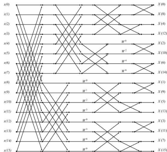
Fig. 14.1.5 Length-16, Decimation-in-Frequency, Split-Radix with special BFs FFT
