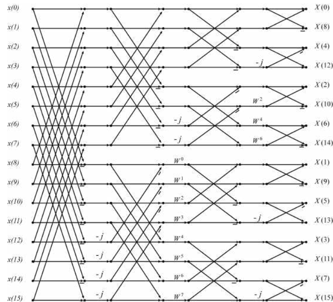
Fig. 14.1.6 Length-16, Decimation-in-Frequency, In-order output, Split-Radix FFT
