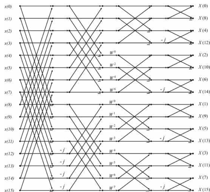
Fig. 14.1.5 Length-16, Decimation-in-Frequency, In-order output, Radix-4 FFT
