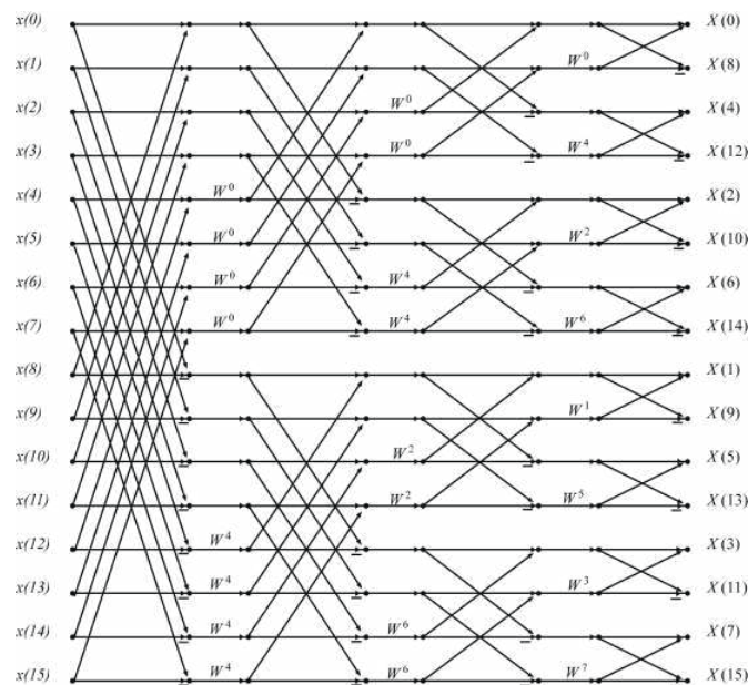
Fig. 14.1.4 Length-16, Decimation-in-Frequency, In-order output, Radix-2 FFT
