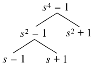
Fig. 6.5.2 Factorization of s^4-1 in steps
