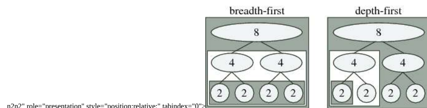
Fig. 10.2.1 Schematic of traditional breadth-first (left) vs. recursive depth-first (right) ordering for radix-2 FFT of size 8: the computations for each n . One ordering distinction is between recursion and iteration. As expressed above, the Cooley-Tukey algorithm could be thought of as defining a tree of smaller and smaller DFTs, as depicted in Fig. 10.2.
