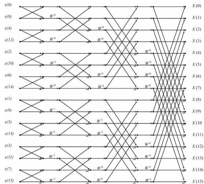
Fig. 14.1.3 Length-16, Decimation-in-Frequency, In-order output, Radix-2 FFT
