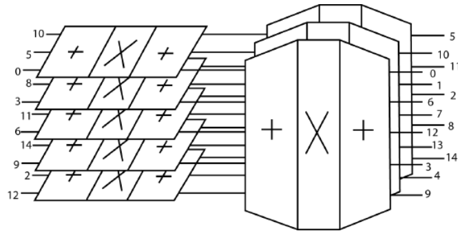
Fig. 9.2.1 A Prime Factor FFT for N = 15
