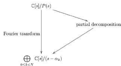
Fig. 7.3.1 Basic idea behind the algebraic derivation of Cooley-Tukey type algorithms
