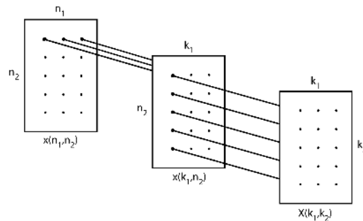
Fig. 2.2.2 Uncoupling of the Row and Column Calculations (Rectangles are Data Arrays)
