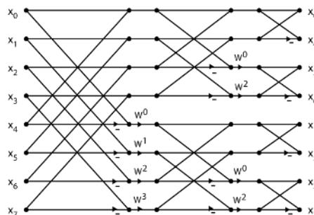
Fig. 8.2.2 Length-8 Radix-2 FFT Flow Graph
