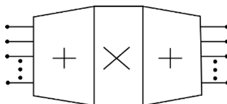
Fig. 6.2.2 Block Diagram of a Winograd Short DFT
