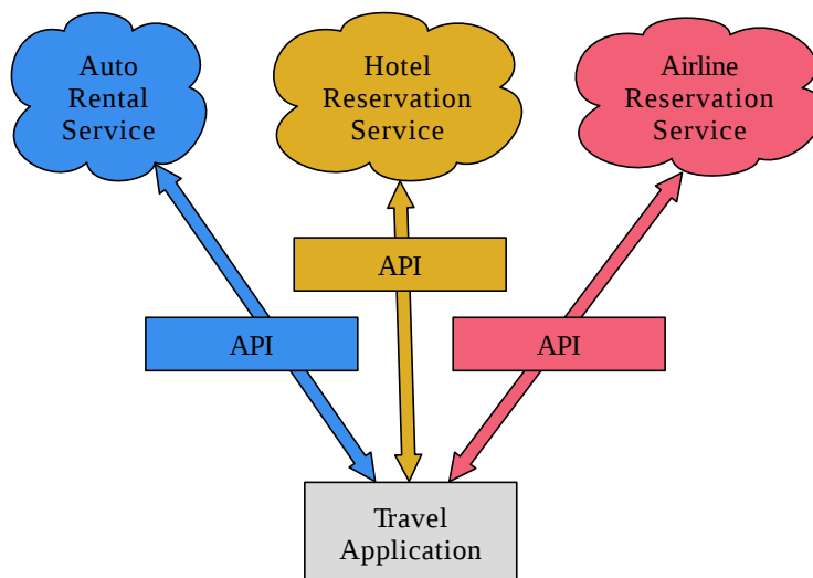
Service Oriented Architecture
