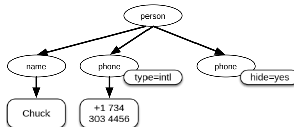
A Tree Representation of XML
