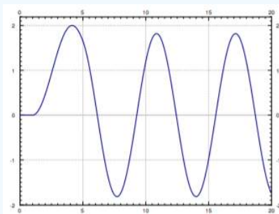
Figure 6.2.2: Plot of x(t) .
