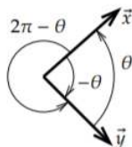
Figure A.5.1: Angle between vectors.
