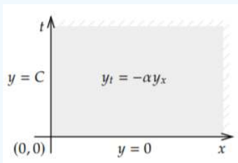
Figure 6.5.1: Transport equation on a half line.
