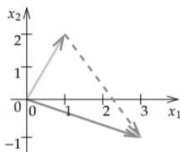
Figure A.1. 2: Adding the vectors (1, 2) , drawn dotted, and (2, -3) , drawn dashed. The result, (3, -1) , is drawn as a solid arrow.
