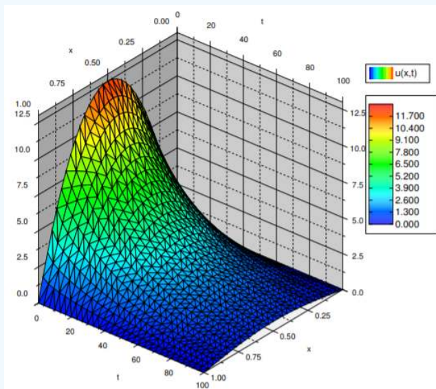
Figure 4.6.3: Plot of the temperature of the wire at position x at time t .
