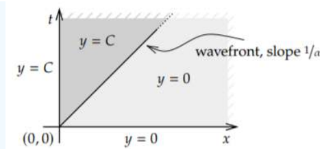
Figure 6.5.2: Wavefront of toxic substance is a line of slope \frac{1}{\alpha} .
