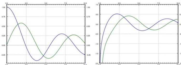
Figure 7.3.1: Plot of the J_0(x) and J_1(x) in the first graph and Y_0(x) and Y_1(x) in the second graph.
