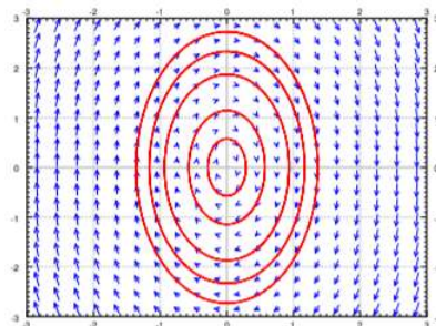
Figure 3.5.6: Example center vector field.
