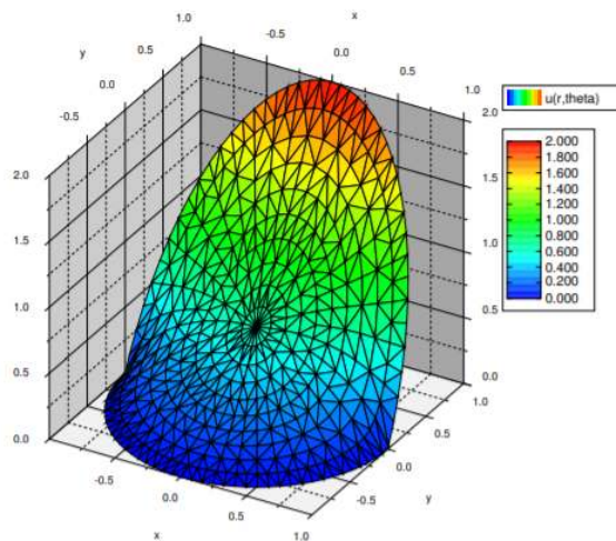
Figure 4.10.4: The solution of the Dirichlet problem with boundary data 0 for y < 0 and 2y for y > 0 .
