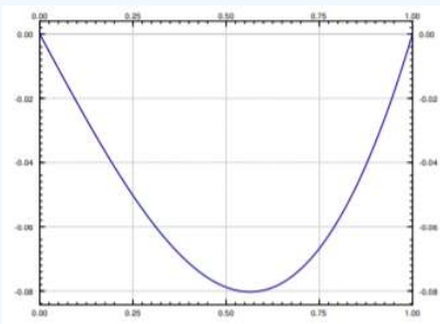
Figure 4.4.2: Plot of the solution of x'' + 2x = t , x(0) = 0 , x(1) = 0 .
