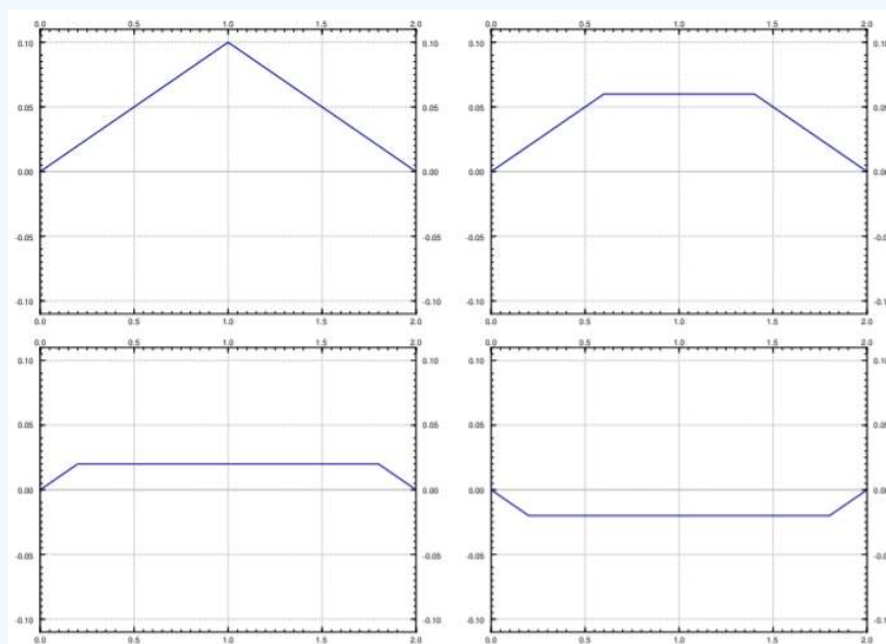
Figure 4.7.4: Plucked string for t = 0 , t = 0.4 , t = 0.8 , and t = 1.2 .
