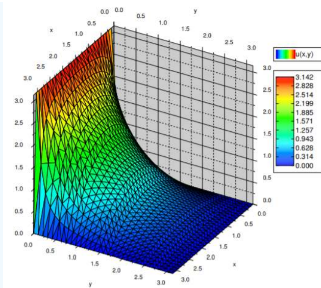
Figure 4.9.2: Steady state temperature of a square plate, three sides held at zero and one side held at \pi .
