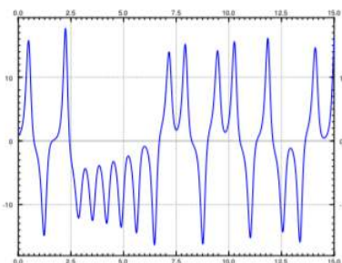
Figure 8.5.6: Graph of the x(t) component of the solution.
