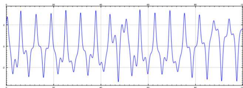
Figure 8.5.3: The solution to the given Duffing equation for t from 0 to 100.
