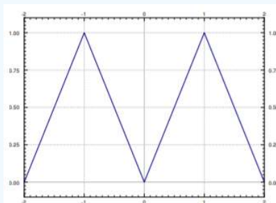
Figure 4.3.1: Periodic extension of the function f(t) .
