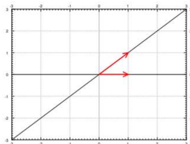
Figure 3.5.2: Eigenvectors of P with directions.
