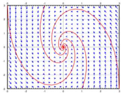
Figure 3.5.8: Example spiral sink vector field.
