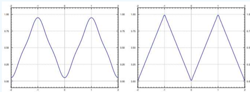
Figure 4.3.2: Fourier series of f(t) up to the 3 rd harmonic (left graph) and up to the 20 th harmonic (right graph).
