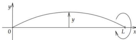
Figure 4.1.1: Whirling string.
