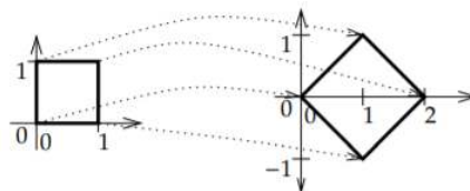
Figure (\PageIndex{1}) : Image of the unit square via the mapping (A) .
