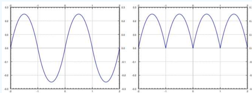
Figure 4.4.1: Odd and even 2-periodic extension of f(t) = t(1-t) , 0 \leq t \leq 1 .
