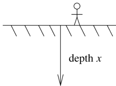
Figure 5.3.3: Underground temperature.
