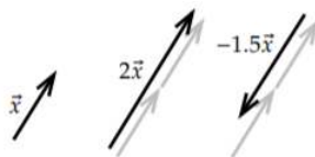
Figure A.1.4: A vector \vec{x} , the vector 2\vec{x} (same direction, double the magnitude), and the vector -1.5\vec{x} (opposite direction, 1.5 times the magnitude).
