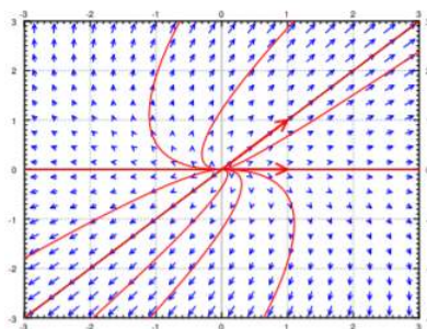
Figure 3.5.3: Example source vector field with eigenvectors and solutions.
