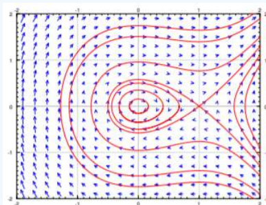
Figure 8.1.2: Phase portrait with some trajectories of x' = y, y' = -x + x^2 .
