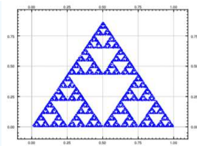
Figure 8.E. 1: 10,000 iterations of the chaos game producing the Sierpinski triangle.
