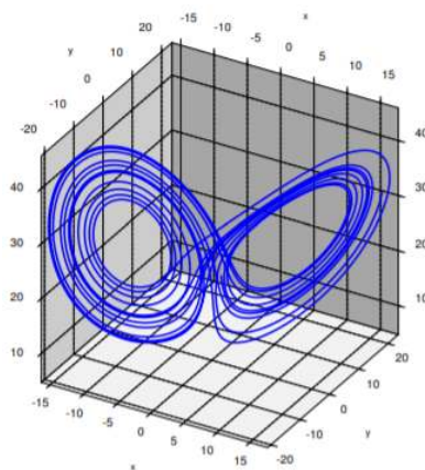
Figure 8.5.5: A trajectory in the Lorenz system.
