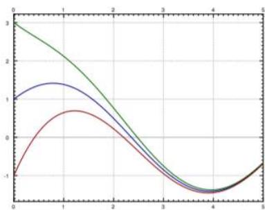
Figure 0.2.1: Few solutions of \frac{dx}{dt} + x = 2 \cos t .
