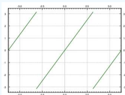
Figure 4.2.2: The graph of the sawtooth function.
