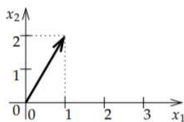
Figure A.1. 1: The vector (1, 2) drawn as an arrow from the origin to the point (1, 2) .
