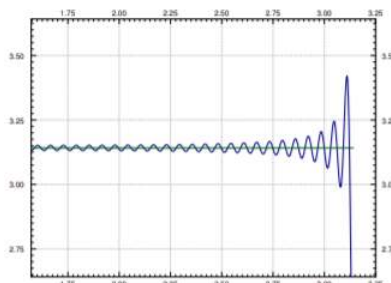
Figure 4.2.6: Gibbs phenomenon in action.
