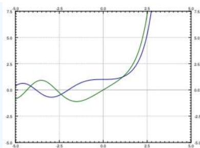
Figure 7.2.1: The two solutions y_1 and y_2 to Airy's equation.
