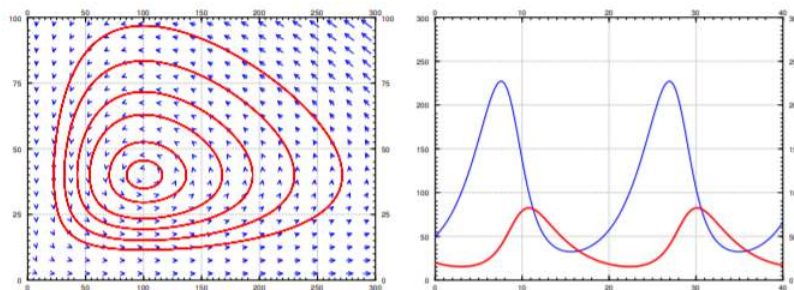
Figure 8.3.5: The phase portrait (left) and graphs of x and y for a sample solution (right).
