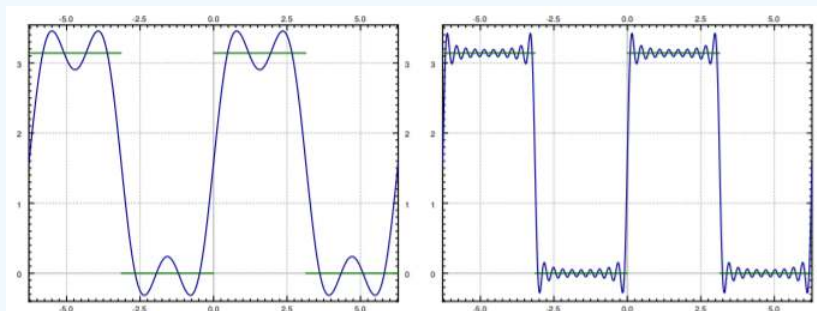
Figure 4.2.5: First 3 (left graph) and 20 (right graph) harmonics of the square wave function.
