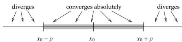
Figure 7.1.1: Convergence of a power series.
