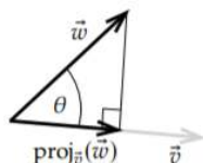
Figure A.5.2: Orthogonal projection.
