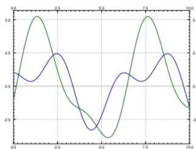
Figure 3.6.4: Superposition of the two modes given the initial conditions.
