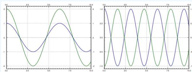
Figure 3.6.3: The two modes of the mass-spring system. In the left plot the masses are moving in unison and in the right plot are masses moving in the opposite direction.
