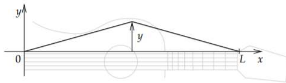
Figure 5.3.1: Vibrating string.
