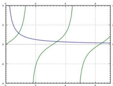
Figure 5.1.1: Plot of \frac{1}{x} and \tan x .
