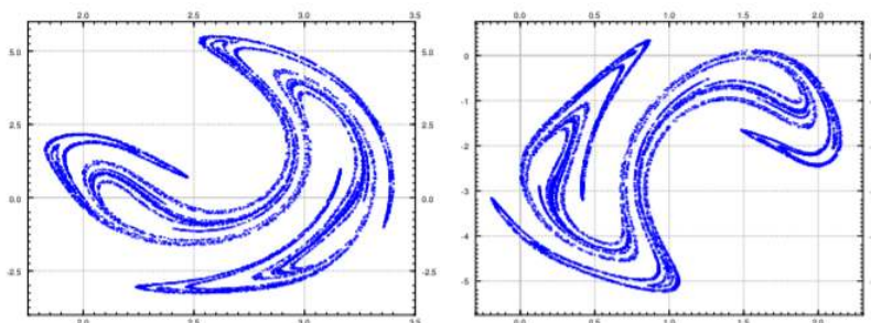
Figure 8.5.4: Strange attractor. The left plot is with no phase shift, the right plot has phase shift \frac{\pi}{4} .
