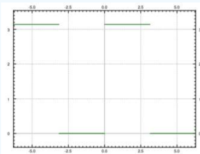
Figure 4.2.4: The graph of the square wave function.
