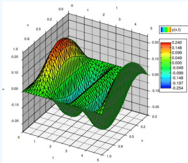
Figure 5.3.2: Plot of y(x, t) = \frac{F(x+t) + F(x-t)}{2} + \left( \cos(x) - \frac{\cos(1) - 1}{\sin(1)} \sin(x) - 1 \right) \cos(t) .
