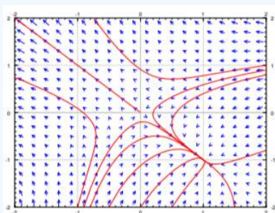
Figure 8.2.1: The phase portrait with few sample trajectories of x' = -y - x^2 , y' = -x + y^2 .
