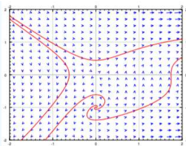
Figure 8.2.2: The phase portrait with few sample trajectories of x' = y + y^2 e^x , y' = x .
