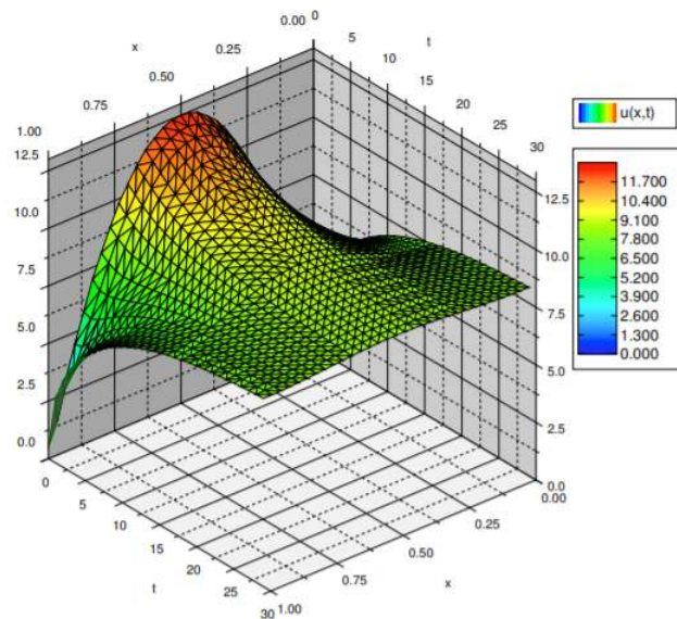
Figure 4.6.5: Plot of the temperature of the insulated wire at position x at time t .
