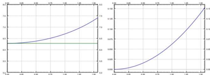
Figure 8.3.4: The plot of T and T_{\text{linear}} with \frac{g}{L} = 1 (left), and the plot of the relative error \frac{T - T_{\text{linear}}}{T} (right), for \theta_0 between 0 and \frac{\pi}{2} .
