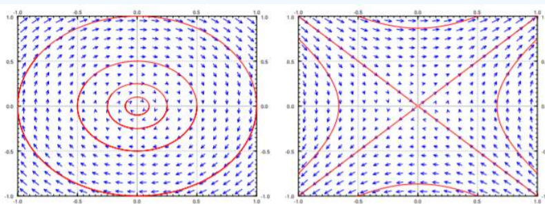
Figure 8.1.3: Phase diagram with some trajectories of linearizations at the critical points (0, 0) (left) and (1, 0) (right) of x' = y , y' = -x + x^2 .
