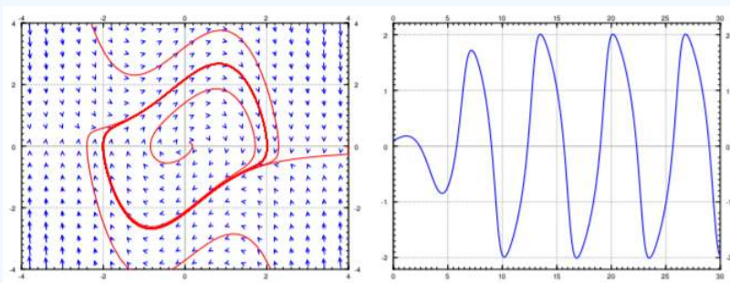
Figure 8.4.1: The phase portrait (left) and a graph of a sample solution of the Van der Pol oscillator.
