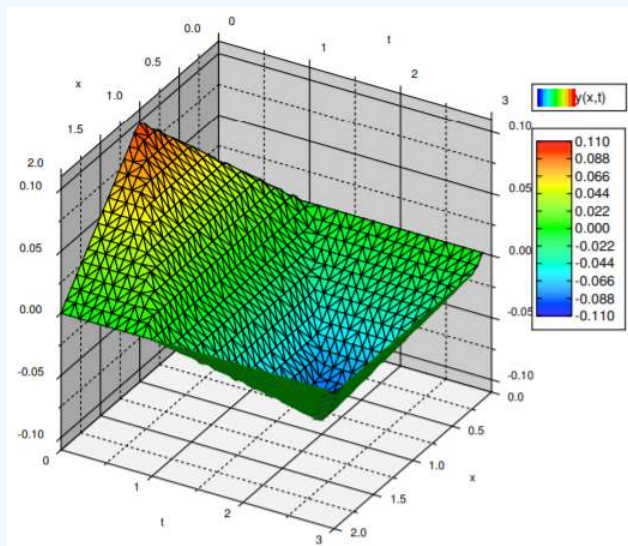
Figure 4.7.3: Shape of the plucked string for 0 < t < 3 .
