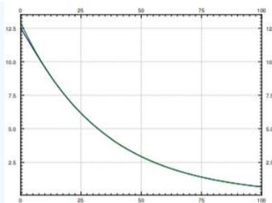
Figure 4.6.4: Temperature at the midpoint of the wire (the bottom curve), and the approximation of this temperature by using only the first term in the series (top curve).
