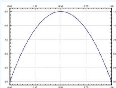
Figure 4.6.2: Initial distribution of temperature in the wire.
