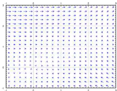
Figure 3.1.3: The direction field for x' = 2y - x, y' = x .
