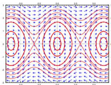
Figure 8.3.2: Phase plane diagram and some trajectories of the nonlinear pendulum equation.
