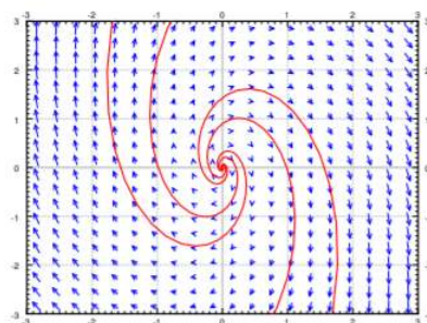
Figure 3.5.7: Example spiral source vector field.
