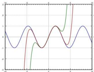
Figure 7.1.2: The sine function and its Taylor approximations around x_0 = 0 of 5 th and 9 th degree.
