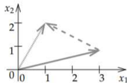
Figure A.1. 3: Subtraction, the vector (1, 2) , drawn dotted, minus (-2, 1) , drawn dashed. The result, (3, 1) , is drawn as a solid arrow.
