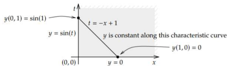
Figure 6.5.3: Ill-posed problem.
