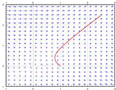
Figure 3.1.4: The direction field for x' = 2y - x, y' = x with the trajectory of the solution starting at (1, 0) for 0 \leq t \leq 2 .
