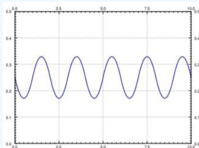
Figure 4.5.1: Plot of the steady periodic solution x_{sp} of Example 4.5.1.
