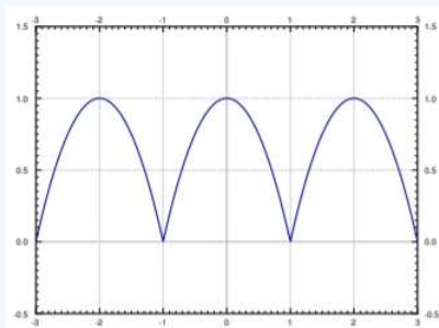
Figure 4.2.1: Periodic extension of the function 1 - t^2 .
