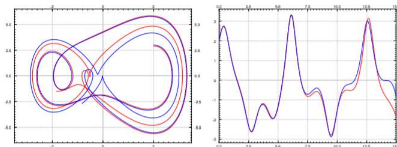
Figure 8.5.2: On left, two trajectories in phase space for 0 \leq t \leq 15 , for the Duffing equation one with initial conditions (2, 3) and the other with (2, 2.9) . On right the two solutions in (x, t) -space.
