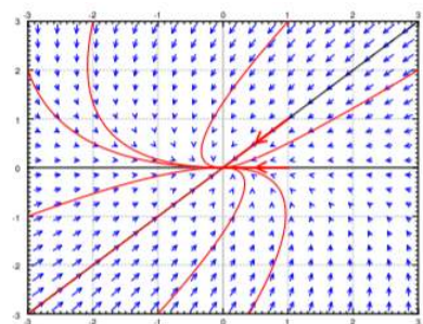
Figure 3.5.4: Example sink vector field with eigenvectors and solutions.
