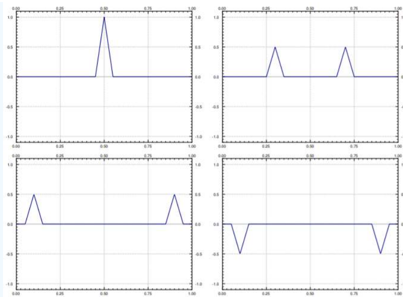
Figure \backslash\text{PageIndex}\{1\} : Plot of the d'Alembert solution for \backslash(t=0\backslash) , \backslash(t=0.2\backslash) , \backslash(t=0.4\backslash) , and \backslash(t=0.6\backslash) .
