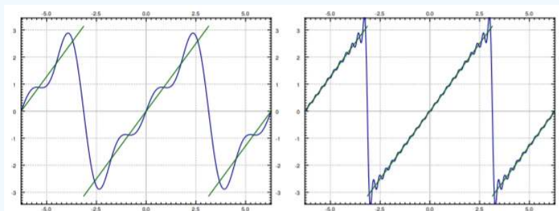
Figure 4.2.3: First 3 (left graph) and 20 (right graph) harmonics of the sawtooth function.
