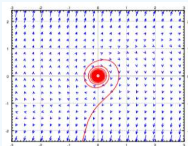
Figure 8.2.3: An unstable critical point (spiral source) at the origin for x' = y , y' = -x + y^3 , even if the linearization has a center.
