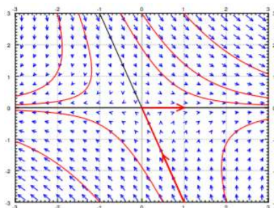
Figure 3.5.5: Example saddle vector field with eigenvectors and solutions.
