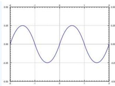
Figure 4.3.3: Smooth 2-periodic function.
