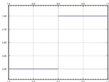
Figure 6.2.1: Plot of the Heaviside (unit step) function u(t) .
