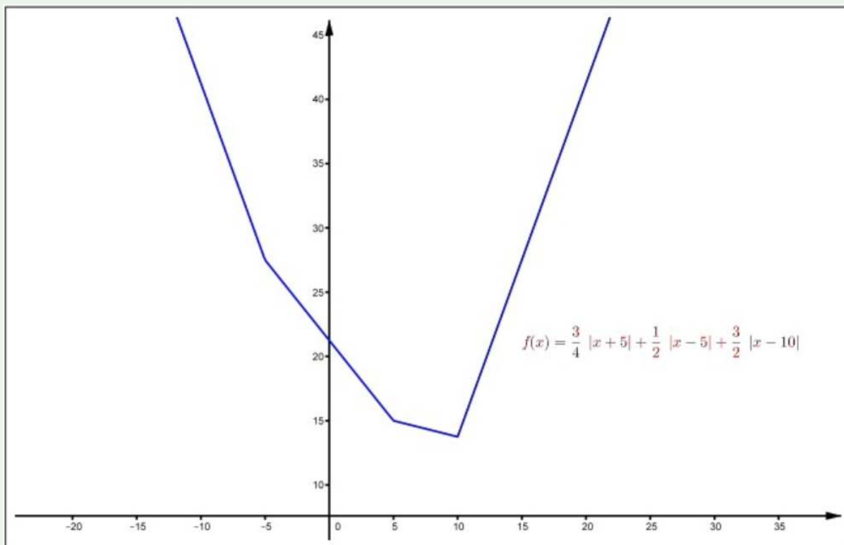
Figure 4.7: A nondifferentiable convex function.
