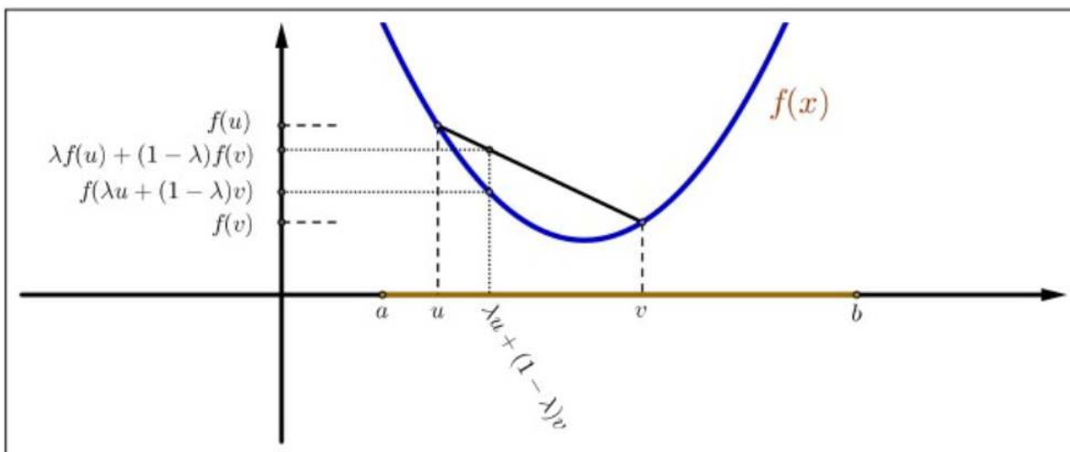
Figure 4.6: A Convex Function.
