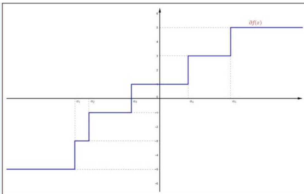
Figure 4.10: Subdifferential of f(x) = \sum_{i=1}^{2k-1} |x - a_i| .
