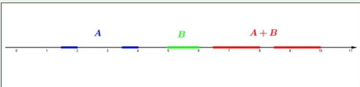
Figure 4.9: Set addition.
