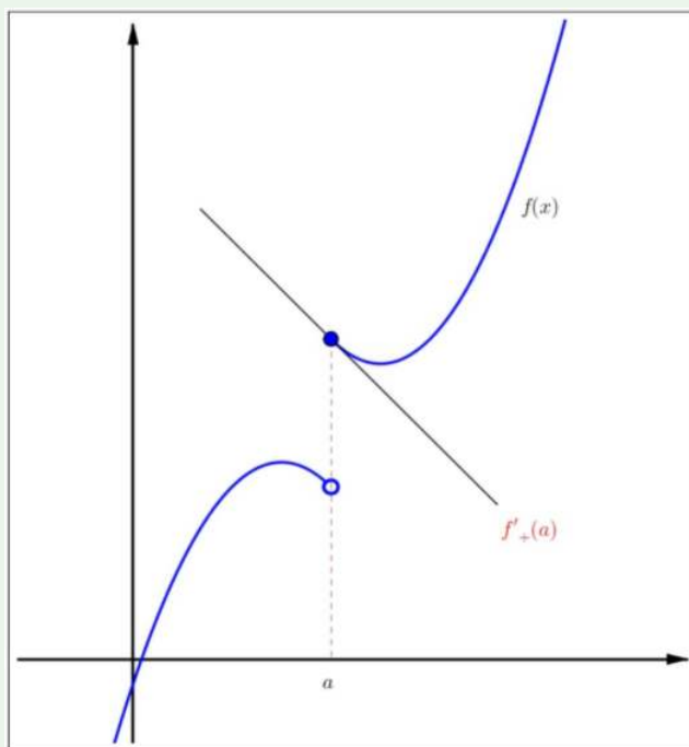
Figure 4.4: Right derivative.
