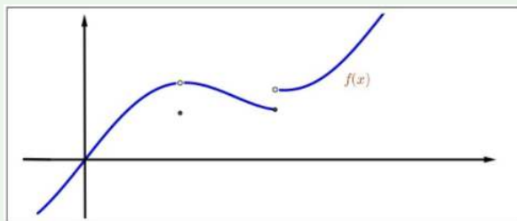
Figure 3.6: Lower semicontinuity.
