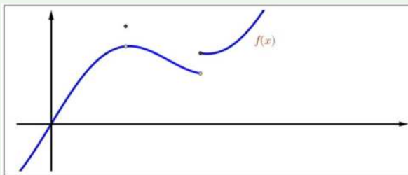
Figure 3.7: Upper semicontinuity.
