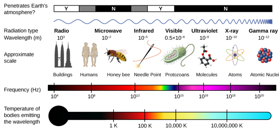
Figure 11.3.1: The electromagnetic spectrum, showing the major categories of electromagnetic waves.
