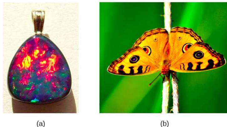
Figure 13.5.4: (a) This Australian opal and (b) butterfly wings have rows of reflectors that act like reflection gratings, reflecting different colors at different angles. (credit a: modification of work by "Opals-On-Black"/Flickr; credit b: modification of work by "whologwhy"/Flickr)
