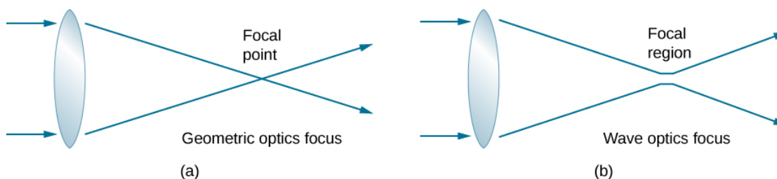
Figure 13.6.7:(a) In geometric optics, the focus is modelled as a point, but it is not physically possible to produce such a point because it implies infinite intensity. (b) In wave optics, the focus is an extended region.
