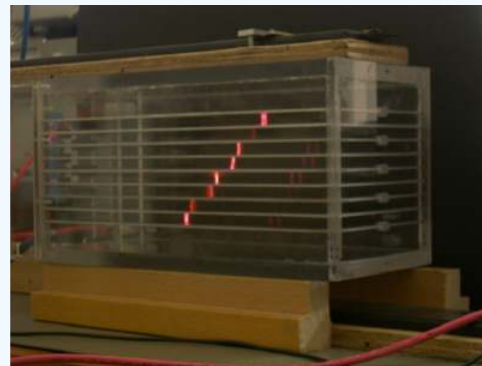
Figure 3.3.5: A spark chamber is used to trace the paths of high-energy particles. Ionization created by the particles as they pass through the gas between the plates allows a spark to jump. The sparks are perpendicular to the plates, following electric field lines between them. The potential difference between adjacent plates is not high enough to cause sparks without the ionization produced by particles from accelerator experiments (or cosmic rays). This form of detector is now archaic and no longer in use except for demonstration purposes. (credit b: modification of work by Jack Collins)
