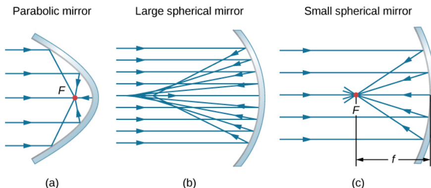
Figure 11.10.3.2: (a) Parallel rays reflected from a parabolic mirror cross at a single point called the focal point F . (b) Parallel rays reflected from a large spherical mirror do not cross at a common point. (c) If a spherical mirror is small compared with its radius of curvature, it better approximates the central part of a parabolic mirror, so parallel rays essentially cross at a common point. The distance along the optical axis from the mirror to the focal point is the focal length f of the mirror.
