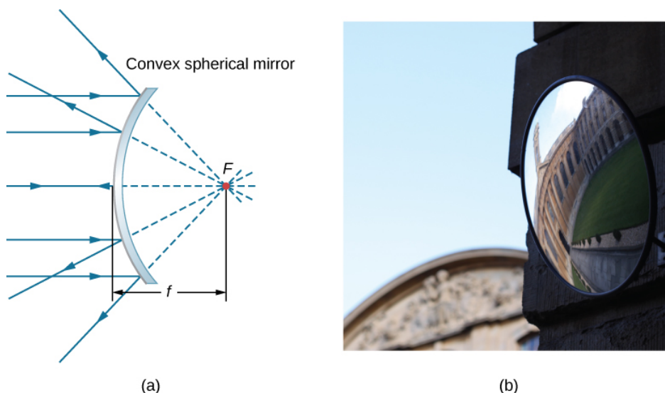
Figure 11.10.3.3: (a) Rays reflected by a convex spherical mirror: Incident rays of light parallel to the optical axis are reflected from a convex spherical mirror and seem to originate from a well-defined focal point at focal distance f on the opposite side of the mirror. The focal point is virtual because no real rays pass through it. (b) Photograph of a virtual image formed by a convex mirror. (credit b: modification of work by Jenny Downing)
