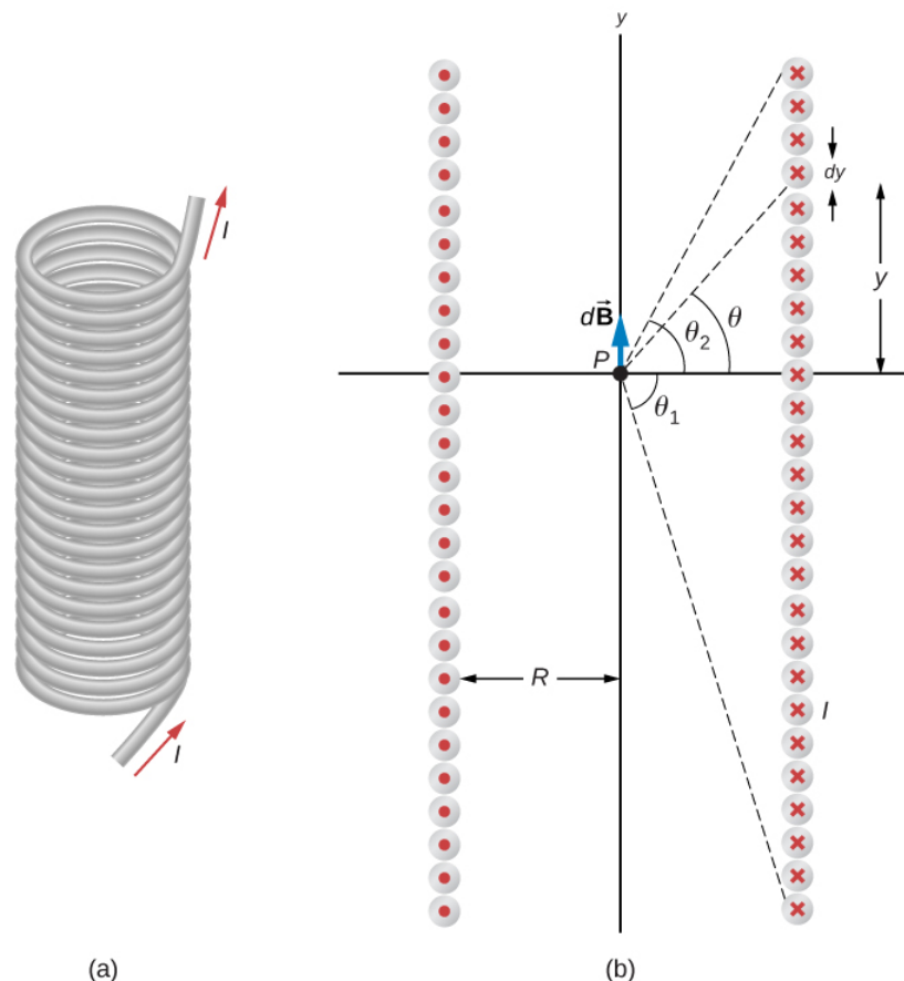
Figure 8.5.2: (a) A solenoid is a long wire wound in the shape of a helix. (b) The magnetic field at the point P on the axis of the solenoid is the net field due to all of the current loops.
