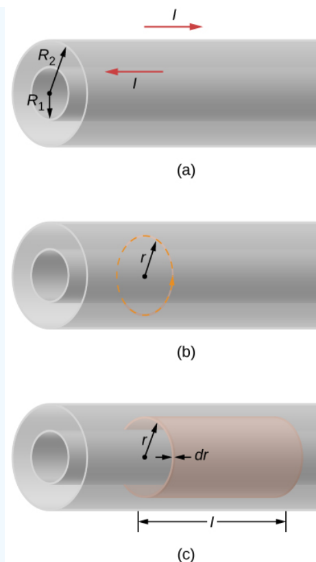
Figure 9.11.1: (a) A coaxial cable is represented here by two hollow, concentric cylindrical conductors along which electric current flows in opposite directions. (b) The magnetic field between the conductors can be found by applying Ampère's law to the dashed path. (c) The cylindrical shell is used to find the magnetic energy stored in a length l of the cable.
