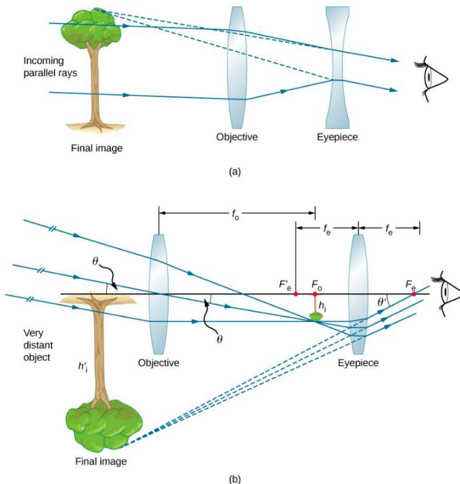
Figure 11.10.9.3: (a) Galileo made telescopes with a convex objective and a concave eyepiece. These produce an upright image and are used in spyglasses. (b) Most simple refracting telescopes have two convex lenses. The objective forms a real, inverted image at (or just within) the focal plane of the eyepiece. This image serves as the object for the eyepiece. The eyepiece forms a virtual, inverted image that is magnified.
