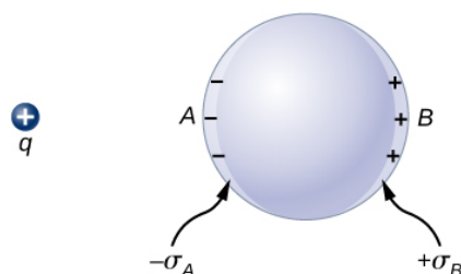
Figure 2.5.1: Polarization of a metallic sphere by an external point charge +q . The near side of the metal has an opposite surface charge compared to the far side of the metal. The sphere is said to be polarized. When you remove the external charge, the polarization of the metal also disappears.
