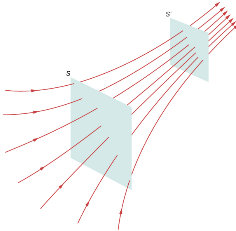
Figure 1.6.4: Electric field lines passing through imaginary areas. Since the number of lines passing through each area is the same, but the areas themselves are different, the field line density is different. This indicates different magnitudes of the electric field at these points.
