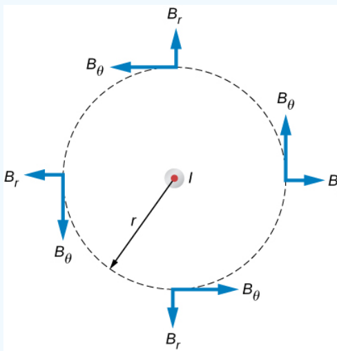
Figure [Math Processing Error] : The possible components of the magnetic field \mathbf{B} due to a current I , which is directed out of the page. The radial component is zero because the angle between the magnetic field and the path is at a right angle.
