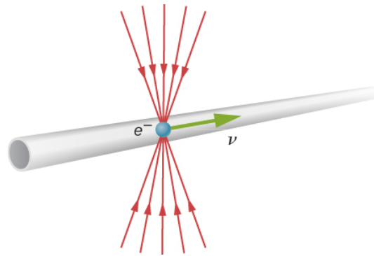
Figure 14.5.5: The electric field lines of a high-velocity charged particle are compressed along the direction of motion by length contraction, producing an observably different signal as the particle goes through a coil.
