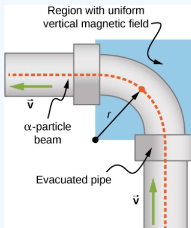
Figure 7.4.4: Top view of the beam deflector setup.
