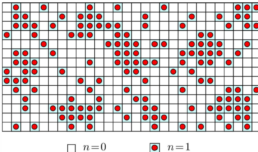
Figure 7.2.1: The lattice gas model. An occupied cell corresponds to n = 1 ( \sigma = +1 ), and a vacant cell to n = 0 ( \sigma = -1 ).
