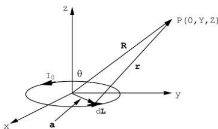
Figure 4.3.9: Calculation of the vector potential generated by a current loop of radius a carrying a current of I_0 Amps.
