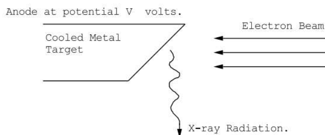
Figure 8.4.4: A schematic diagram of an X-ray tube illustrating the production of the white X-ray spectrum. The electrons undergo a de-acceleration upon striking the metal anode. This de-acceleration is of order a = 1024 \text{ m/sec}^2 for a typical 20 keV potential drop between the anode and the cathode: this assumes an electron stopping distance of 35 \times 10^{-10} \text{ m} . During a brief period, \sim 10^{-16} seconds, the electron radiates at the rate of \sim 5.7 \times 10^{-6} \text{ Watts} , therefore each electron emits a pulse of radiation containing \sim 5.7 \times 10^{-22} \text{ Joules} . The number of electrons that impinge on the anode per second for a beam of 1 mAmp is 6.25 \times 10^{15} . The average power in the X-ray beam will be (6.25 \times 10^{15})(5.7 \times 10^{-22}) = 3.6 \times 10^{-6} \text{ Watts} . This energy is distributed over a range of frequencies from zero to 4.8 \times 10^{18} \text{ Hz} ( h\nu_{\max} = |e|V ). This calculation does not include the energy contained in the characteristic X-ray spectrum emitted from the target.
