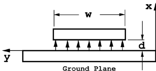
Figure 11.1.2: A strip-line. E_x = E_0 , V = E_0 d , H_y = E_0/Z_0 , I = wJ_s = w(E_0/Z_0)
