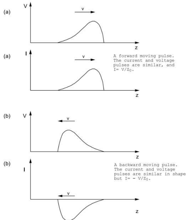
Figure 11.2.5: Voltage and current pulses on a transmission line.
