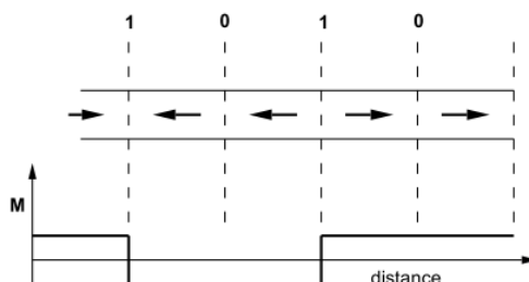
Figure 6.3.12: Example of encoded data bits on a hard disc drive.
