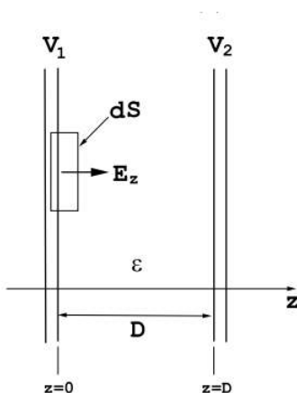
Figure 3.2.2: Two plane parallel, semi-infinite metal electrodes separated by a distance D . The electrode potentials are V_1 and V_2 . The space between the electrodes is filled with a material having a dielectric constant \epsilon .
