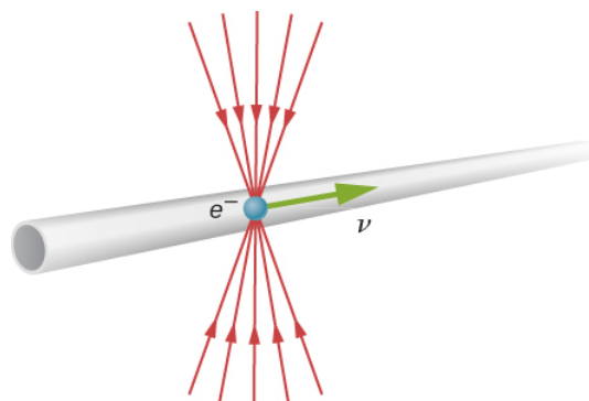
Figure 5.5.5: The electric field lines of a high-velocity charged particle are compressed along the direction of motion by length contraction, producing an observably different signal as the particle goes through a coil.
