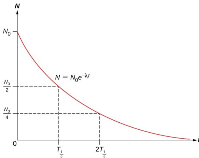
Figure 10.4.2: A plot of the radioactive decay law demonstrates that the number of nuclei remaining in a decay sample drops dramatically during the first moments of decay.
