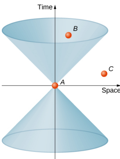
Figure 5.6.3: The light cone consists of all the world lines followed by light from the event A at the vertex of the cone.
