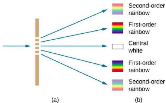
Figure 4.5.3: (a) Light passing through a diffraction grating is diffracted in a pattern similar to a double slit, with bright regions at various angles. (b) The pattern obtained for white light incident on a grating. The central maximum is white, and the higher-order maxima disperse white light into a rainbow of colors.
