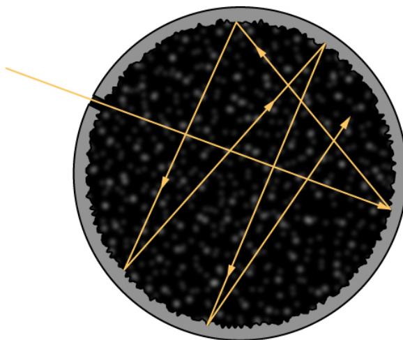
Figure 6.2.1: A blackbody is physically realized by a small hole in the wall of a cavity radiator.
