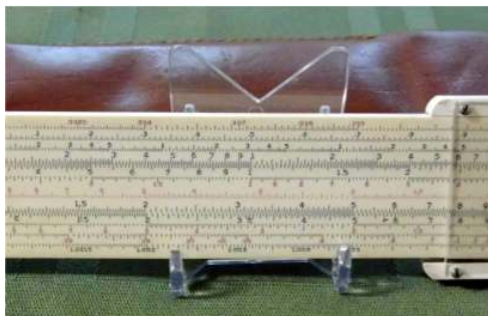
Figure 12.1.1b: Slide Ruler
