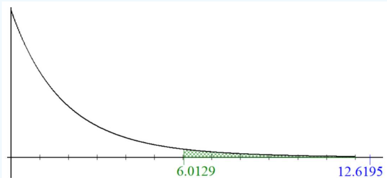
Figure 11-2: Sampling distribution curve with the critical value and calculated F-value shown.
