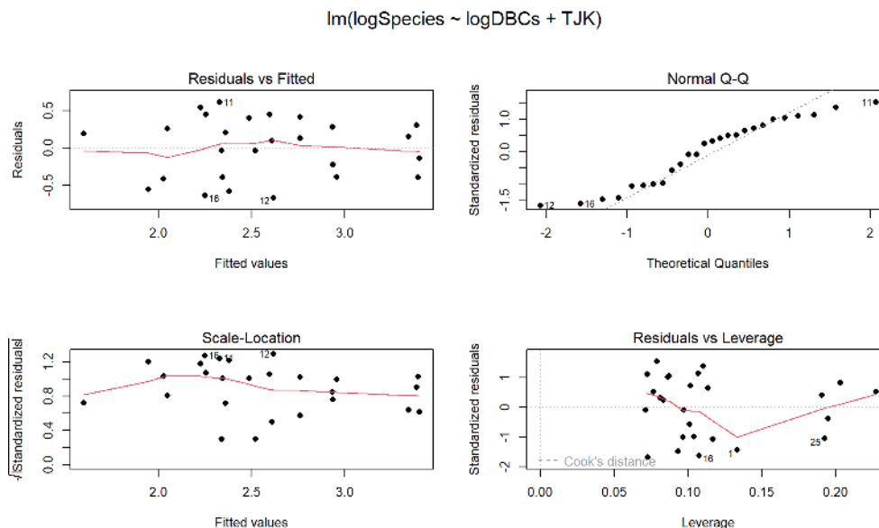
Figure 9.11: Diagnostic plots for the top AIC model.
