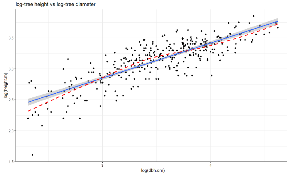
Figure 7.16: Scatterplot of \log(\text{tree height}) versus \log(\text{tree diameter}) .
