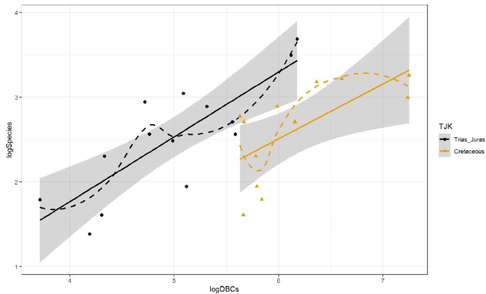
Figure 9.10: Scatterplot of log-biodiversity vs log-DBCs by TJK .
