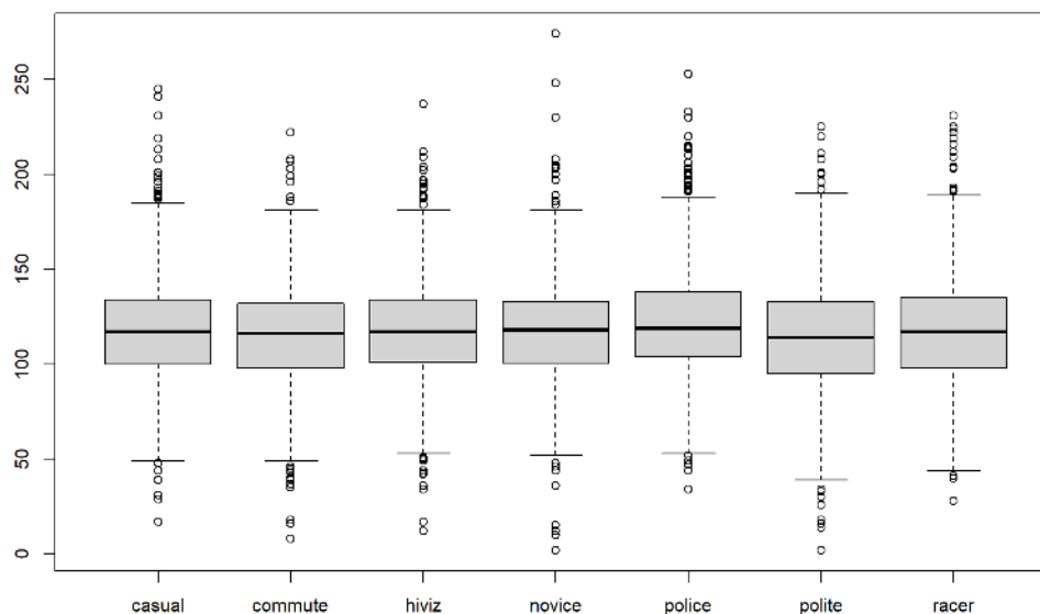
Figure 2.3: Side-by-side boxplot of distances based on outfits.
