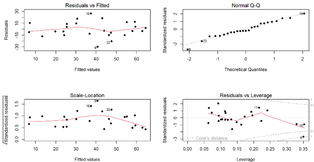
Figure 8.6: Diagnostic plots for model m4: \text{Snow.Depth} \sim \text{Elevation} + \text{Min.Temp} + \text{Max.Temp} .
