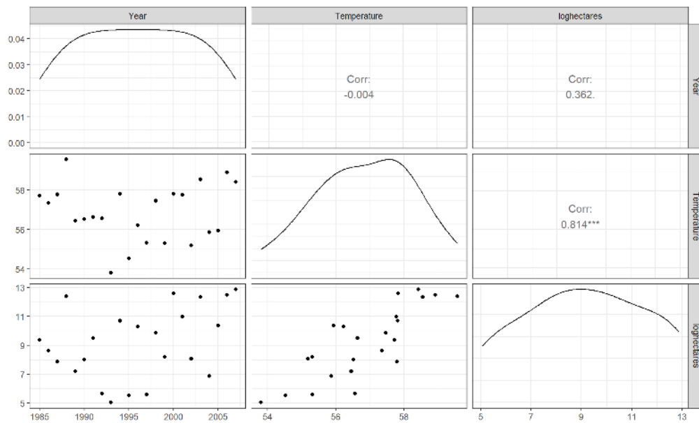
Figure 6.3: Scatterplot matrix of Montana fires data.
