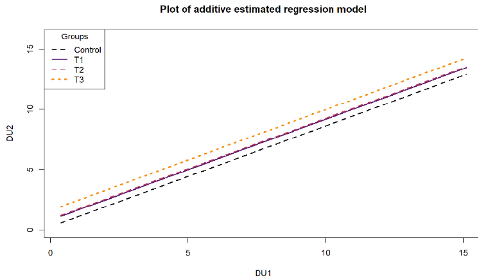
Figure 8.27: Plot of estimated noise tolerance additive model.
