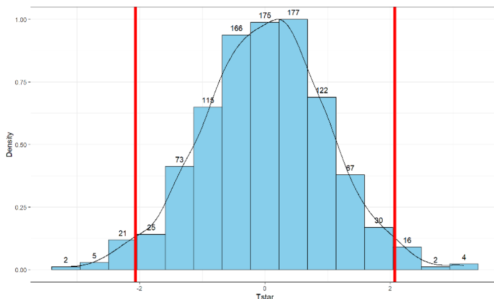
Figure 2.12: Permutation distribution of the t -statistic.
