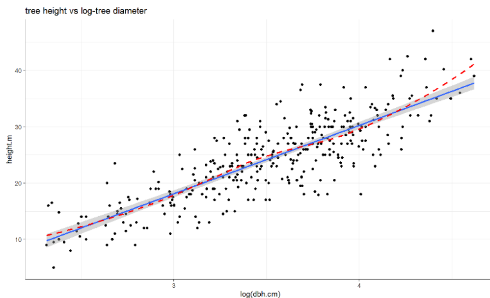
Figure 7.15: Scatterplot of tree height versus log(tree diameter).
