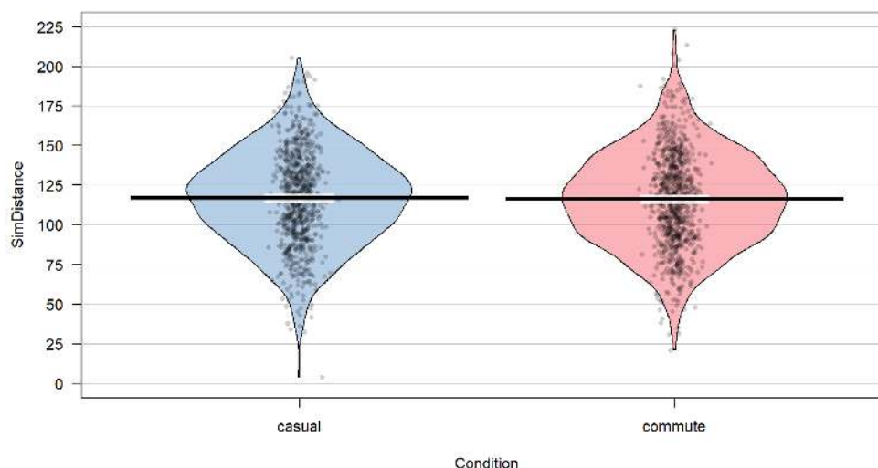
Figure 2.18: Violin-plot of a simulated data set that assumes the same mean for both groups. The means in the two groups are very similar.
