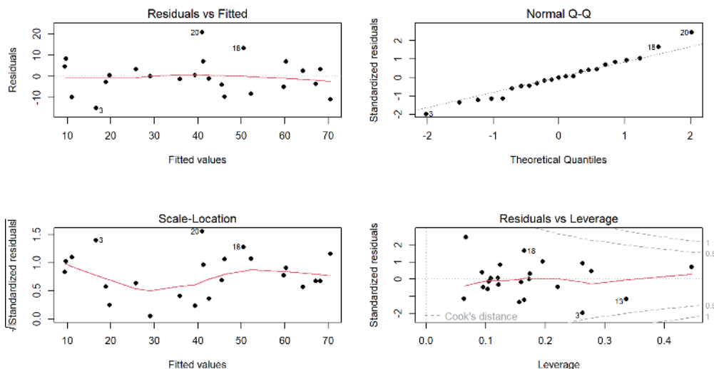
Figure 8.9: Diagnostic plots for MLR for Snow Depth based on Elevation, Min Temp and Max Temp with two observations removed ( n = 23 ).
