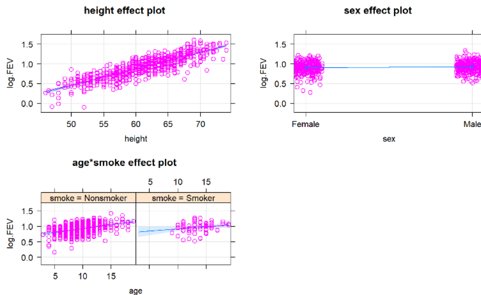
Figure 8.44: Term-plots for the log(FEV) model that includes height, sex, and an interaction between age and smoking status (the full model), with partial residuals.
