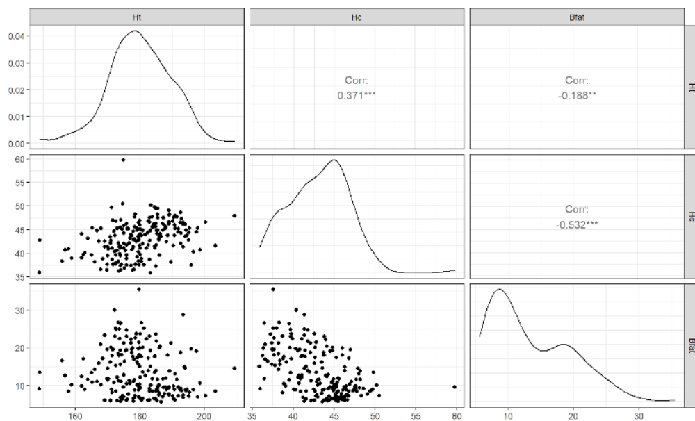
Figure 6.4: Scatterplot matrix of athlete data.
