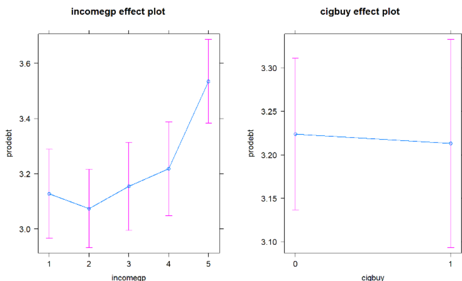
Figure 4.19: Term-plots for the prodebt response additive model with left panel for income group and the right panel for buying cigarettes or not (0 for no, 1 for yes).
