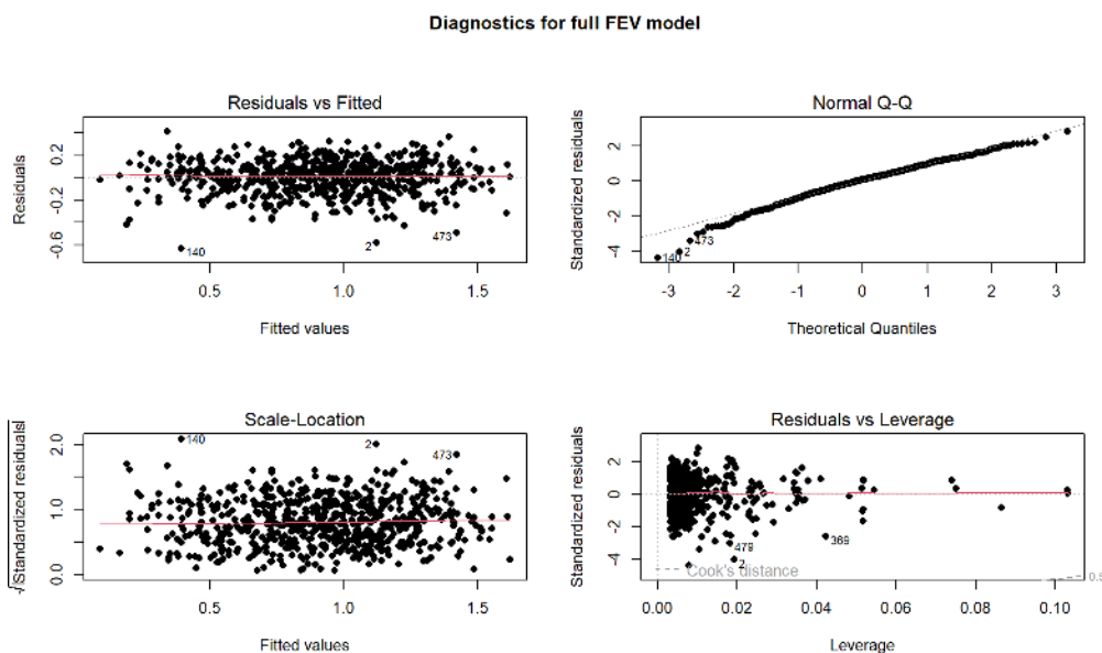
Figure 8.43: Diagnostics for the log(FEV) model that includes height, sex, and an interaction between age and smoking status (the full model).
