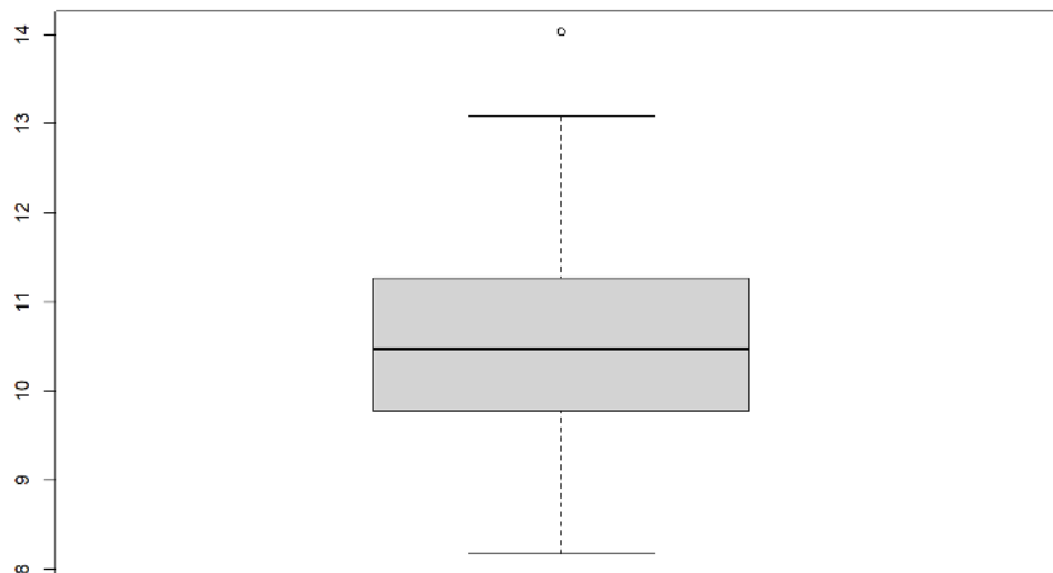
Figure 1.8: Boxplot of 1.5 mile Run Times.
