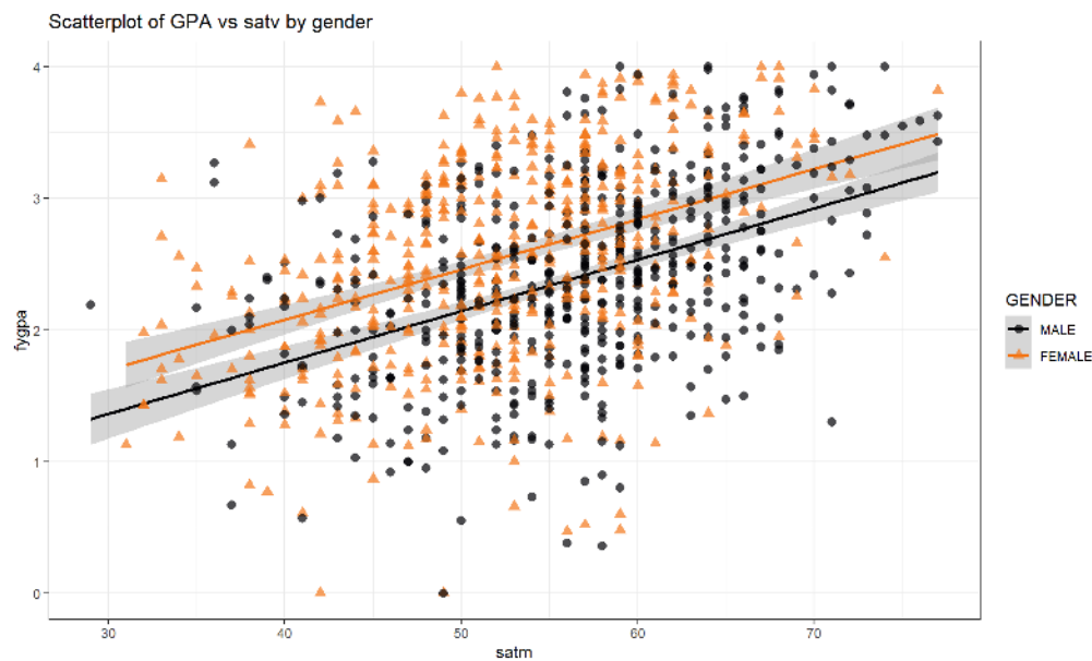
Figure 8.23: Plot of fygpa vs satm by gender of students.
