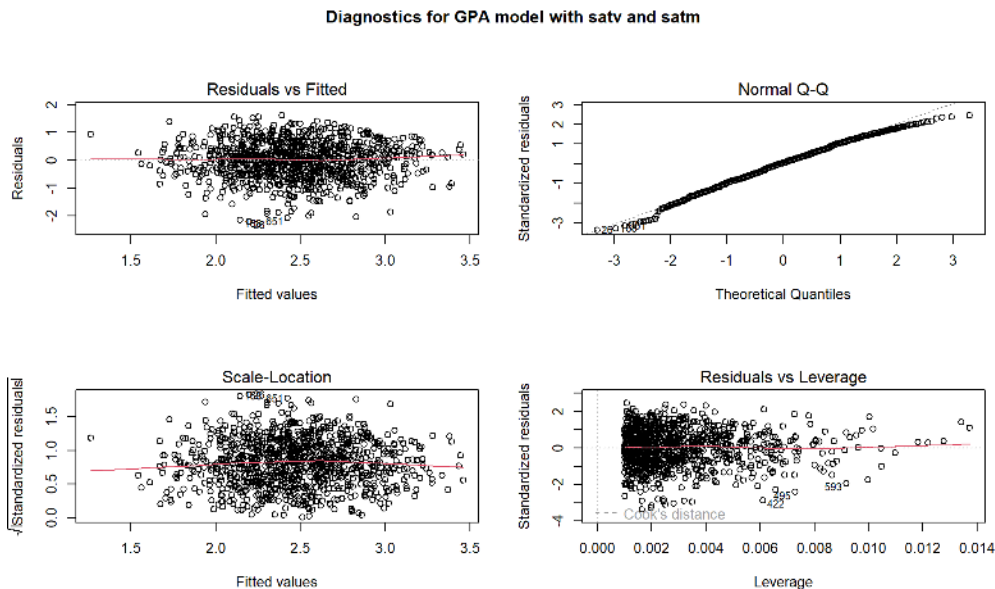
Figure 8.19: Diagnostic plots for the \text{fygpa} \sim \text{satm} + \text{satv} model.
