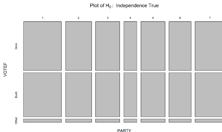
Figure 5.6: Mosaic plot of what the 2000 election data would look like if the null hypothesis of no relationship were true.
