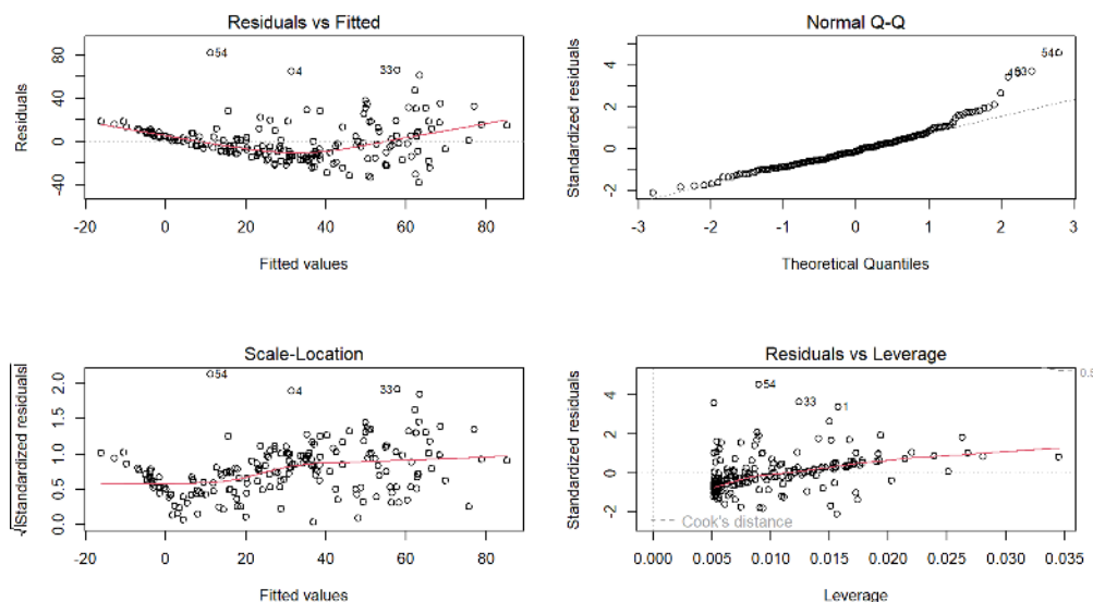
Figure 7.20: Diagnostics plots of the infant mortality model with log(GDP).
