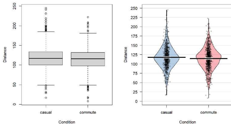
Figure 2.5: Boxplot and pirate-plot of the Distance responses on the reduced ddsub data set.
