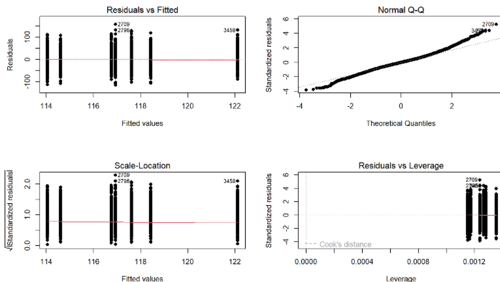
Figure 3.9: Default diagnostic plots for the full overtake data linear model.
