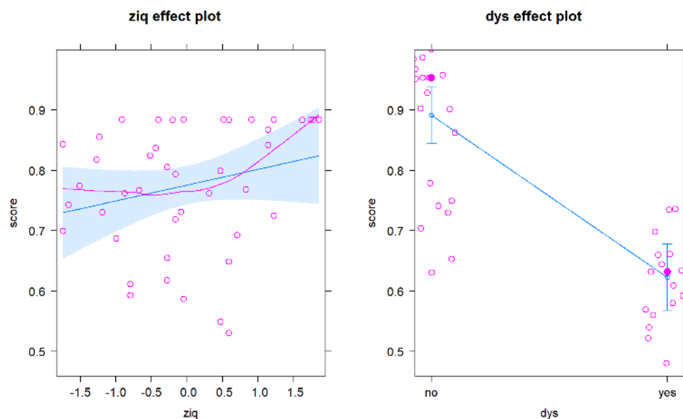
Figure 8.36: Term-plots for additive model for reading scores.
