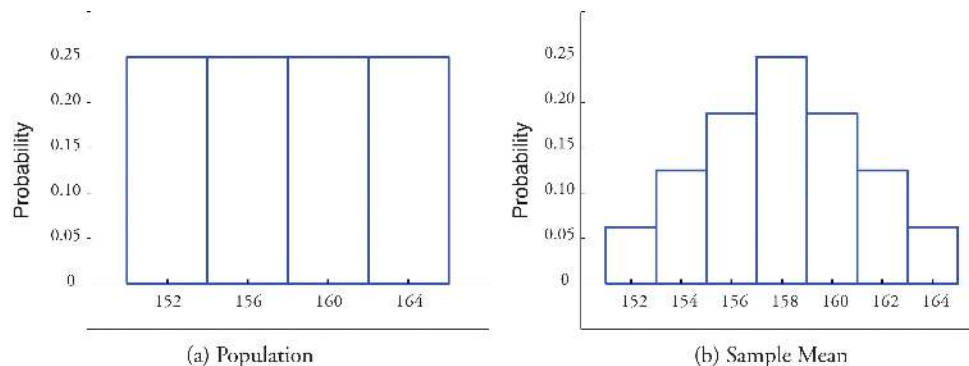
Figure 7.2.1: Distribution of a Population and a Sample Mean
