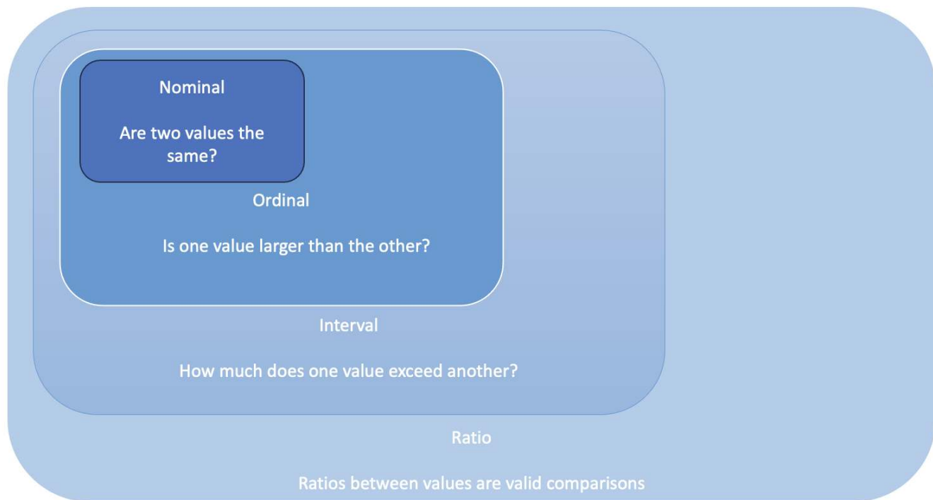
Figure 5.3.1: The relationship between the different types of measurement scales. (Public domain image created by Alan M. Polansky)
