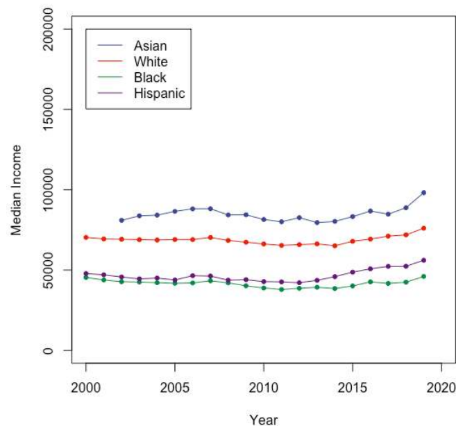
Figure 11.5.4: Line graph of income by race from 2000–2019 based on data obtained from Wilson (2020) using an expanded vertical axis (Public domain image created by Alan M. Polansky)
