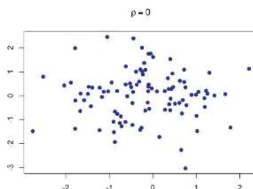
Figure 13.3.1: Scatterplot of data from two variables with the linear strength association with correlation coefficient \rho = 0.00 . (Public domain image created by Alan M. Polansky)
