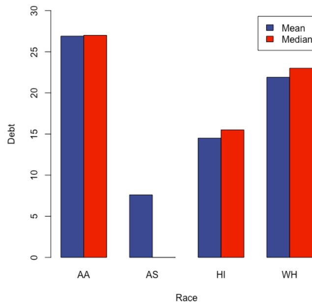
Figure 11.3.4: Graph of a side-by-side bar graph for mean (blue) and median (red) debt by race. Information given in Table 10.2 (Public domain image created by Alan M. Polansky).
