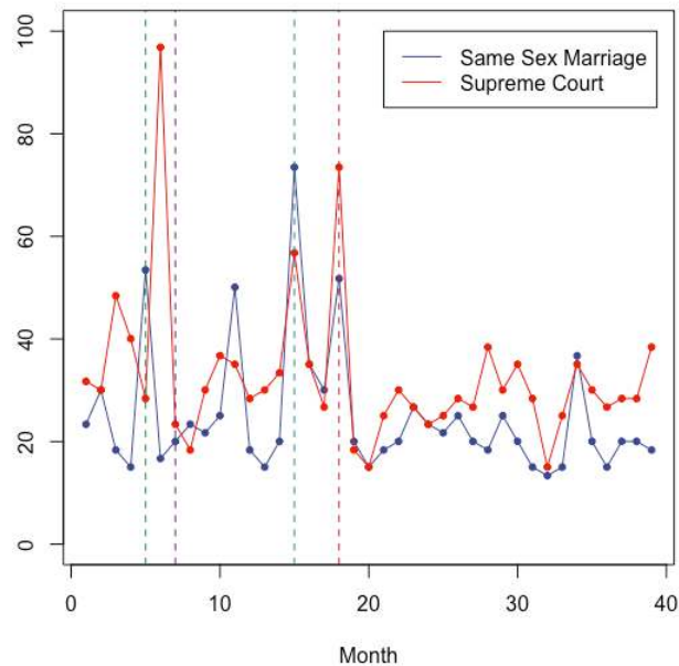
Figure 11.5.2: Line graph of National trends in Google information searching on “same-sex marriage” (blue) and “United States Supreme Court” (red). The green dashed line indicates when President Obama announced support for same sex marriage. The purple dashed line indicates when the Affordable Care Act was upheld by the Supreme Court. The teal dashed line indicates when oral arguments were heard on same sex marriage, and the red dashed line indicates when the final court ruling was announced. The first month indicated on the plot corresponds to February 2012. The plot is adapted from information contained in (Flores and Barclay 2016). (Public domain image created by Alan M. Polansky).
