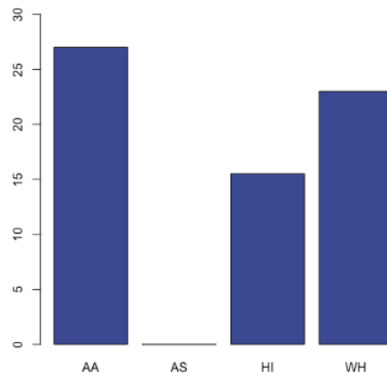
Figure 11.3.2: Bar graph of median debt by race information given in Table 10.2 (Public domain figure created by Alan M. Polansky).
