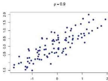
Figure 13.3.7: Scatterplot of data from two variables with the linear strength association with correlation coefficient \rho = 0.90 . (Public domain image created by Alan M. Polansky)
