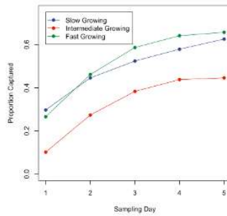
Figure 11.8.1.3: The cumulative proportion of fish captured in the third lake for slow-, intermediate-, and fast-growing fish adapted from Biro (2013). (Public domain image created by Alan M. Polansky)
