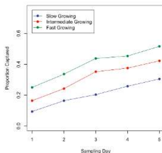
Figure 11.8.1.2: The cumulative proportion of fish captured in the second lake for slow-, intermediate-, and fast-growing fish adapted from Biro (2013). (Public domain image created by Alan M.Polansky)
