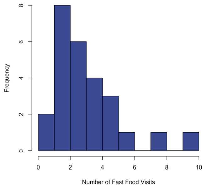
Figure 11.6.1: Number of times people said they ate at fast-food restaurants in the last week (Public domain image created by Alan M. Polansky)
