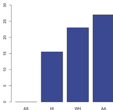
Figure 11.3.3: Bar graph of median debt by race information given in Table 10.2 (Public domain figure created by Alan M. Polansky).
