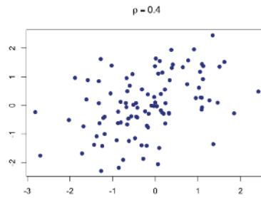
Figure 13.3.3: Scatterplot of data from two variables with the linear strength association with correlation coefficient \rho = 0.40 . (Public domain image created by Alan M. Polansky)
