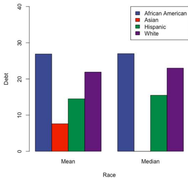
Figure 11.3.5: Graph of a side-by-side bar graph for African American (blue), Asian (red), Hispanic (green), and white (purple). Information given in Table 10.2 (Public domain image created by Alan M. Polansky).
