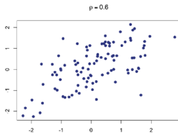
Figure 13.3.5: Scatterplot of data from two variables with the linear strength association with correlation coefficient \rho = 0.60 . (Public domain image created by Alan M. Polansky)
