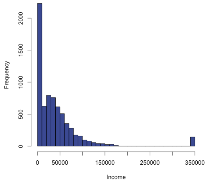
Figure 11.6.5: The incomes of 7,006 individuals extracted from the National Longitudinal Study, which is sponsored by the U.S. Bureau of Labor Statistics (Public domain image created by Alan M. Polansky)
