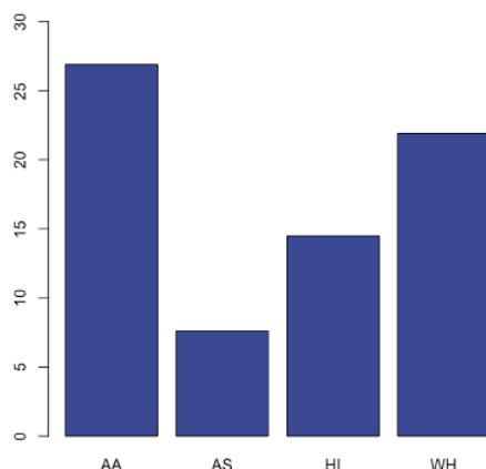
Figure 11.3.1: Bar graph of mean debt by race information given in Table 10.2 (Public domain figure created by Alan M. Polansky).
