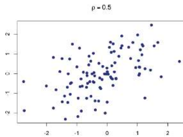
Figure 13.3.4: Scatterplot of data from two variables with the linear strength association with correlation coefficient \rho = 0.50 . (Public domain image created by Alan M. Polansky)
