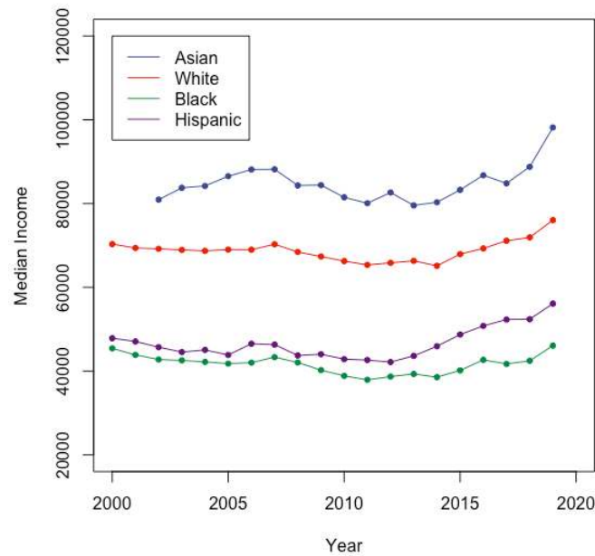
Figure 11.5.3: Line graph of income by race from 2000–2019 based on data obtained from Wilson (2020) (Public domain image created by Alan M. Polansky)
