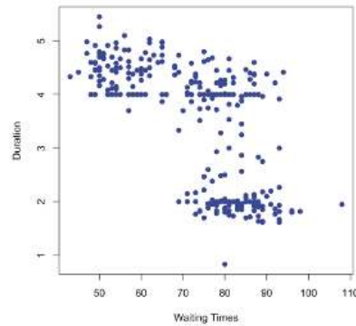
Figure 11.7.2: Observations of the time interval between and the subsequent duration of eruptions of the geyser Old Faithful in Yellowstone National Park, Wyoming, United States from Azzalini and Bowman (1990) (Public domain image created by Alan M. Polansky)
