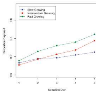
Figure 11.8.1.1: The cumulative proportion of fish captured in the first lake for slow-, intermediate-, and fast-growing fish adapted from Biro (2013). (Public domain image created by Alan M.Polansky)
