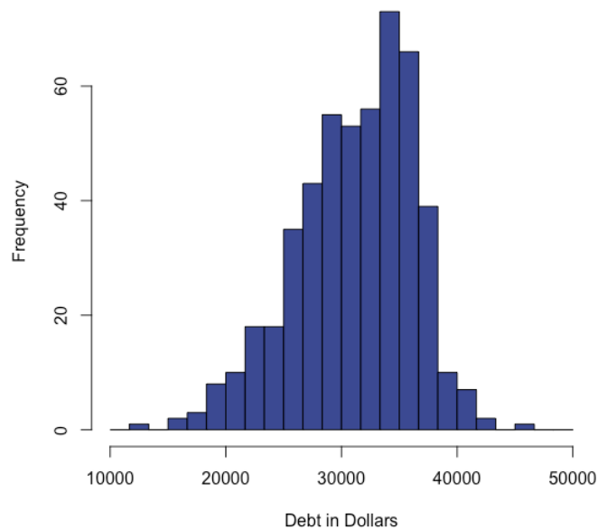
Figure 11.6.4: Histogram of simulated student loan debt (Public domain image created by Alan M. Polansky)
