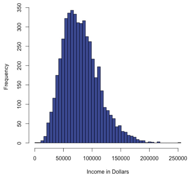
Figure 11.6.3: Histogram of simulated incomes (Public domain image created by Alan M. Polansky)
