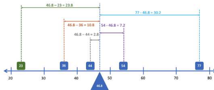
Figure 9.4.1: Computing the absolute deviations for the data from the example. The vertical dashed line indicates the location of the data as measured by the mean. The absolute deviations are indicated by the distances between each point and the mean (Public domain figure created by Alan M. Polansky).
