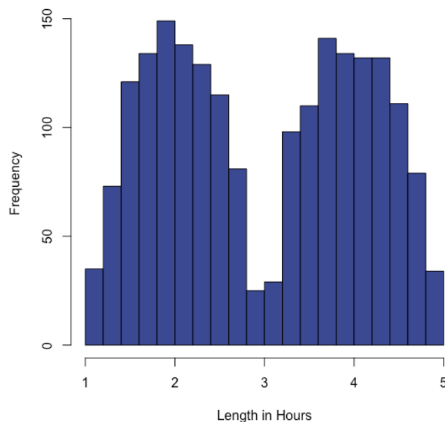
Figure 11.6.2: Histogram of simulated headache lengths for those taking a pain reliever, and those who took a placebo (Public domain image created by Alan M. Polansky)
