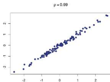
Figure 13.3.8: Scatterplot of data from two variables with the linear strength association with correlation coefficient \rho = 0.99 . (Public domain image created by Alan M. Polansky)
