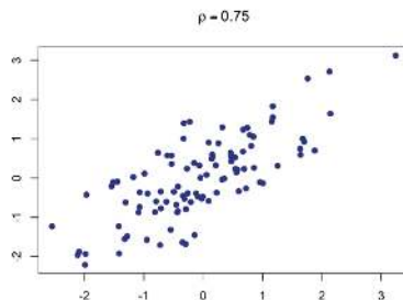
Figure 13.3.6: Scatterplot of data from two variables with the linear strength association with correlation coefficient \rho = 0.75 . (Public domain image created by Alan M. Polansky)
