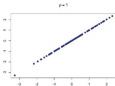
Figure 13.3.9: Scatterplot of data from two variables with the linear strength association with correlation coefficient \rho = 1.00 . (Public domain image created by Alan M. Polansky)
