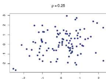
Figure 13.3.2: Scatterplot of data from two variables with the linear strength association with correlation coefficient \rho = 0.25 . (Public domain image created by Alan M. Polansky)
