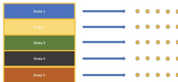
Figure 8.5.2: A graphical depiction of stratified sampling. The population has been divided into five strata. From each strata a simple random sample of individuals is taken. (Public domain image created by Alan M. Polansky)
