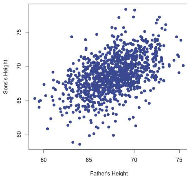
Figure 11.7.1: The height of 1,078 sons' heights plotted against their fathers' heights, a dataset studied by the famous statistician Karl Pearson in 1903. Both measurements are in inches (Public domain image created by Alan M. Polansky)
